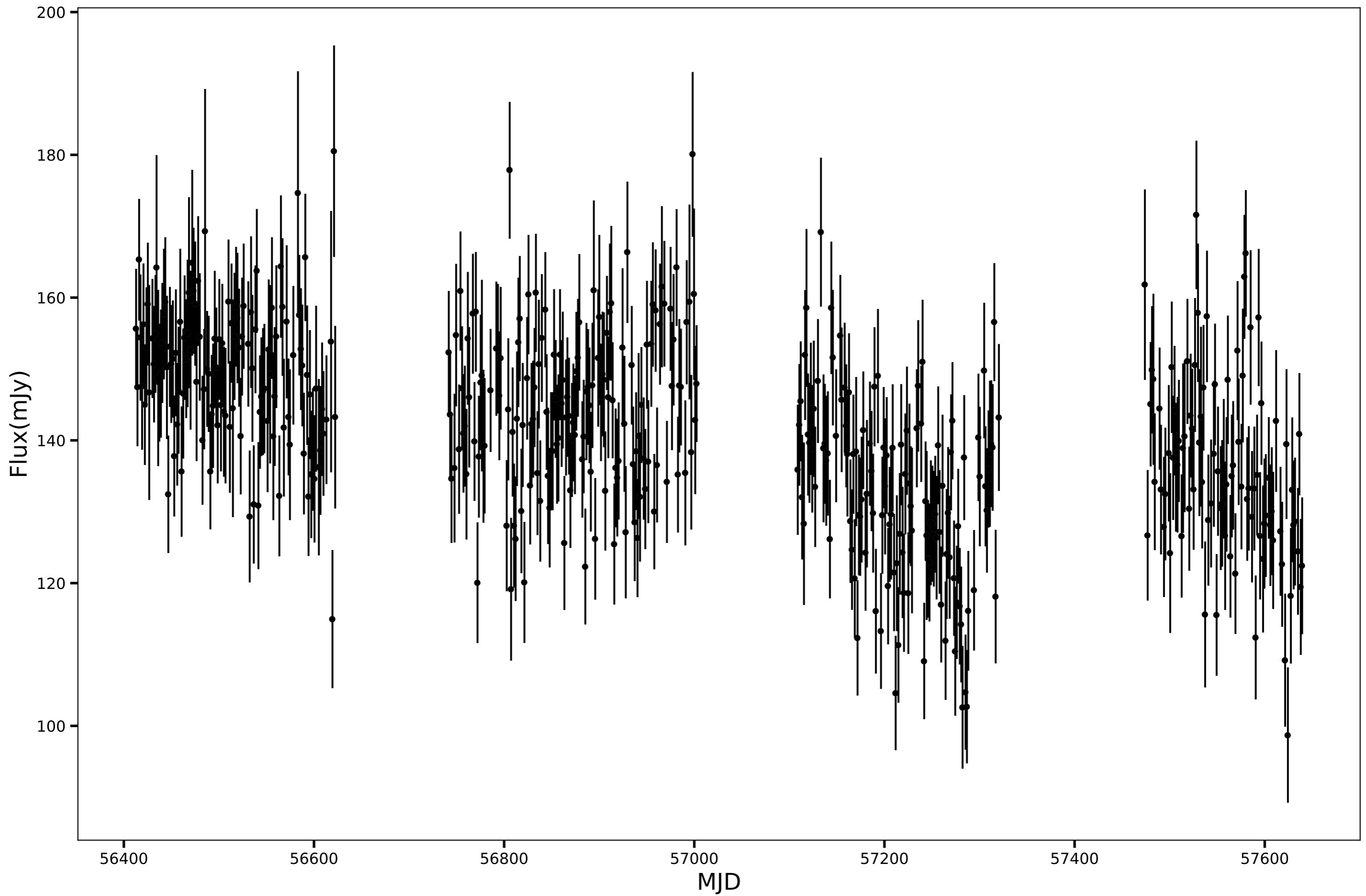
SPT-SJ235844-6053.0, RA=359.6871d, DEC=-60.8845d, mean_flux=141.21 (mJy)
