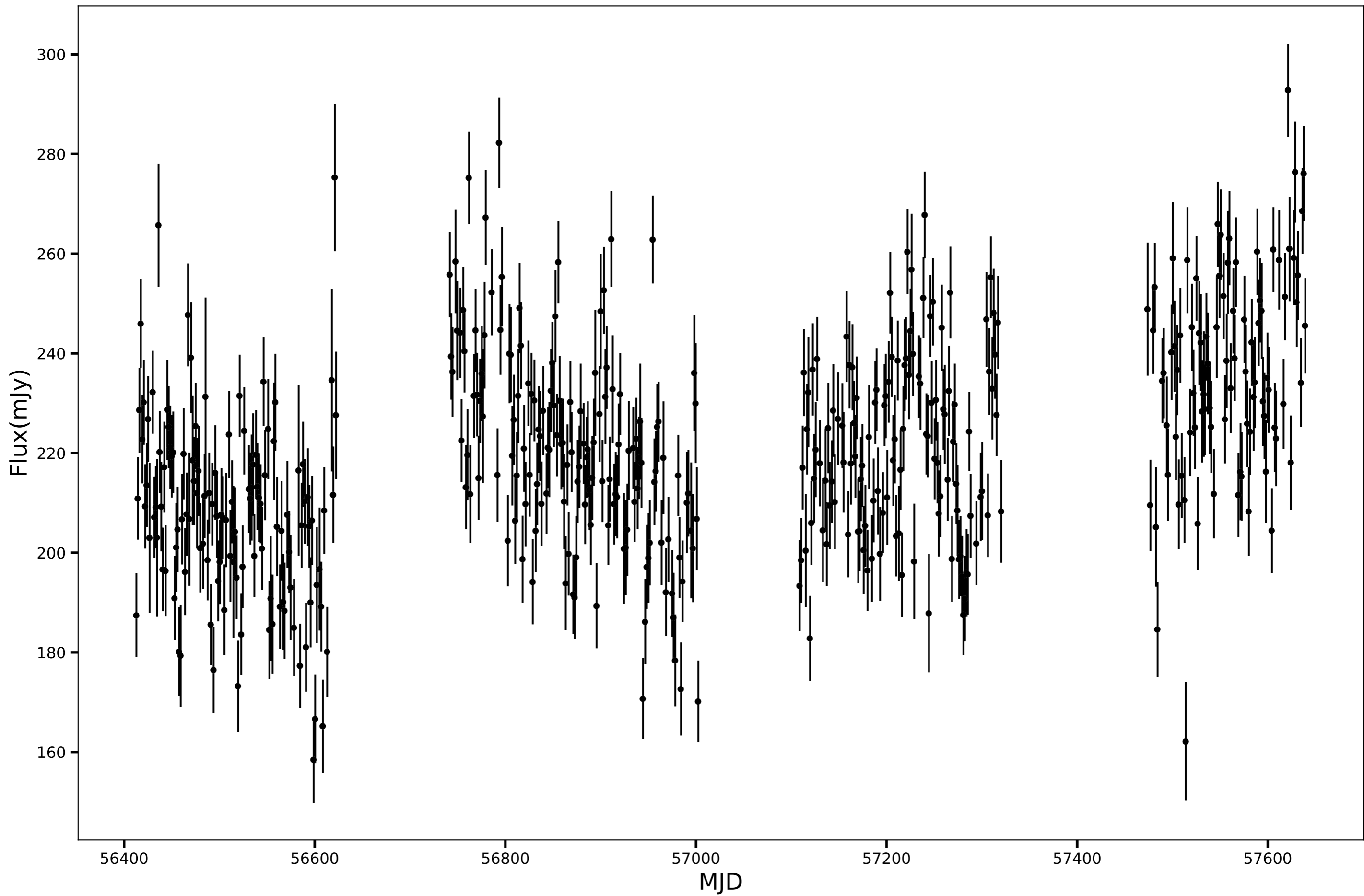
SPT-SJ234925-4932.4, RA=357.3583d, DEC=-49.5408d, mean_flux=220.58 (mJy)
