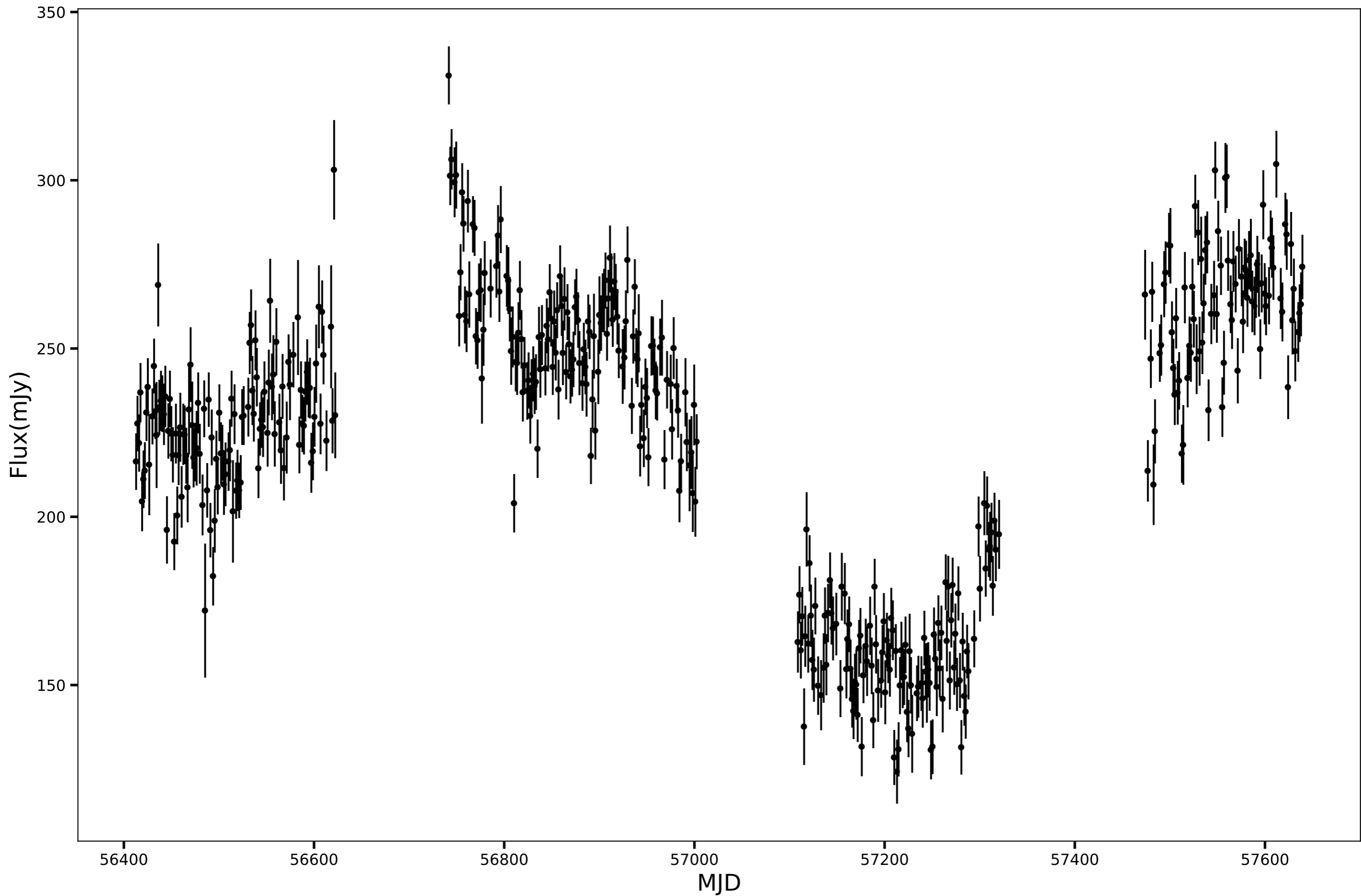
SPT-SJ234720-5110.6, RA=356.8338d, DEC=-51.1769d, mean_flux=224.75 (mJy)
