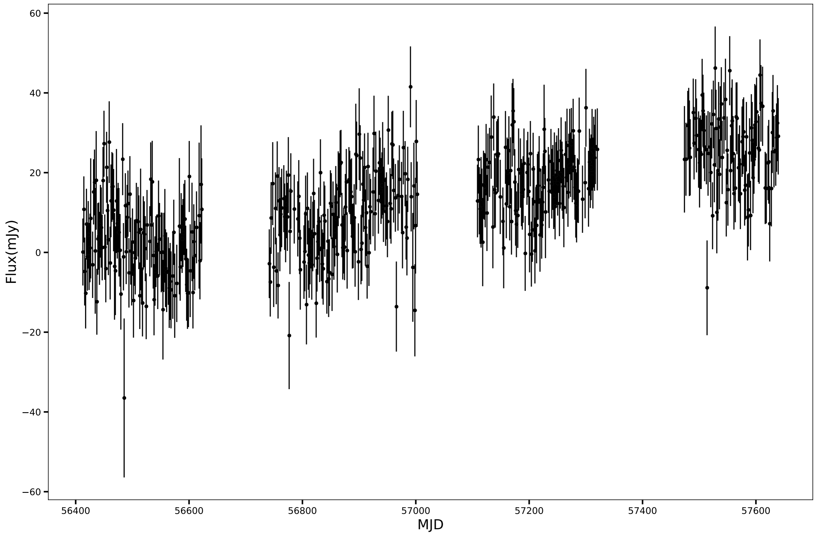
SPT-SJ233913-5523.7, RA=354.8046d, DEC=-55.3963d, mean_flux=12.76 (mJy)
