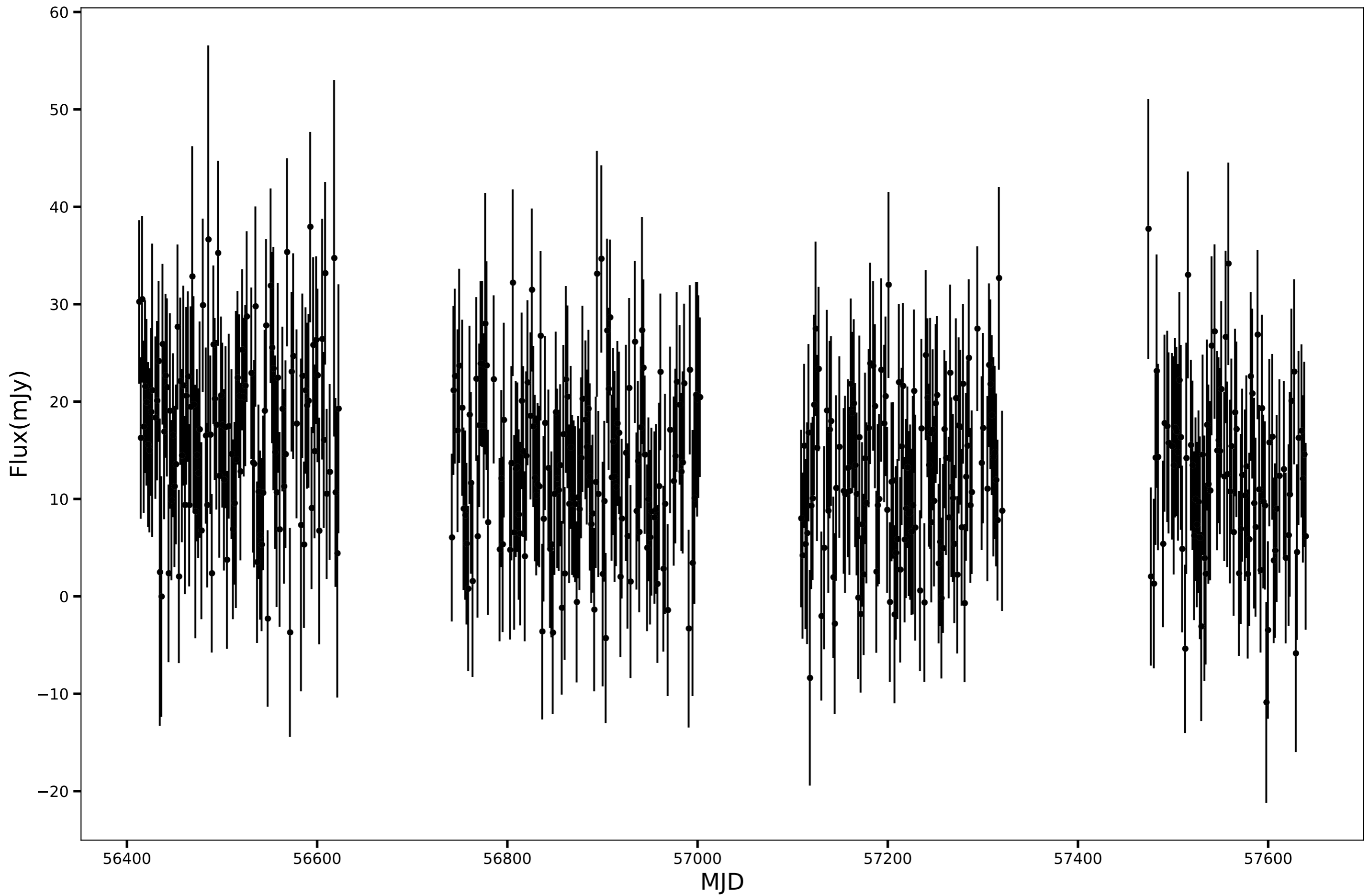
SPT-SJ232510-5656.4, RA=351.2957d, DEC=-56.9409d, mean_flux=13.97 (mJy)
