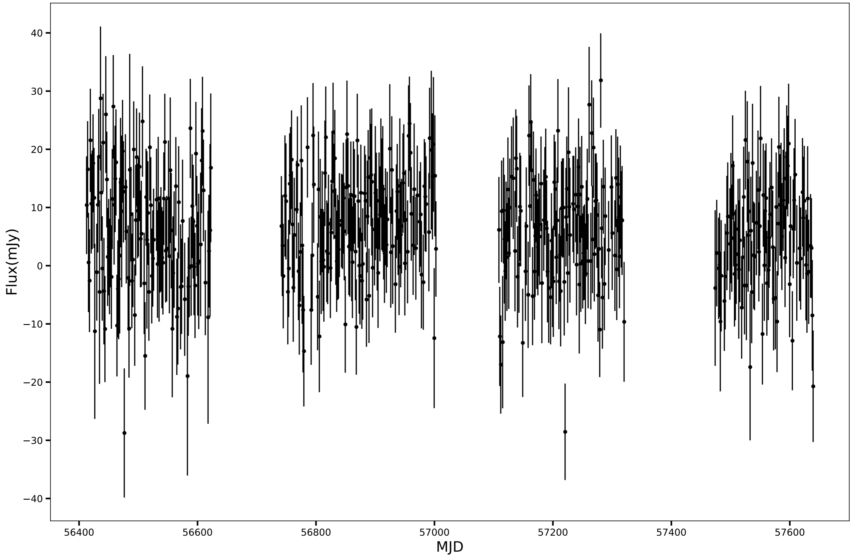
SPT-SJ230159-5343.4, RA=345.4991d, DEC=-53.7236d, mean_flux=6.06 (mJy)
