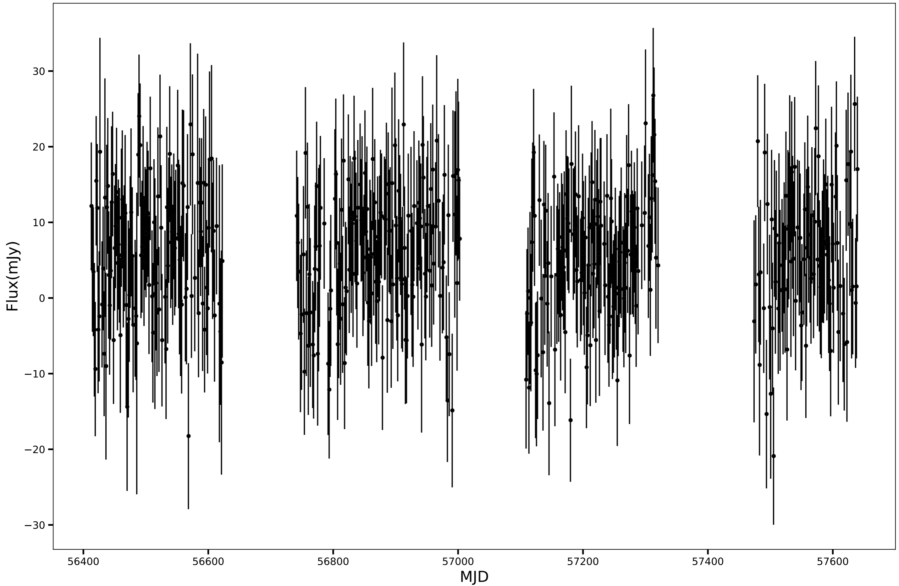
SPT-SJ225858-5919.9, RA=344.7449d, DEC=-59.3328d, mean_flux=5.60 (mJy)
