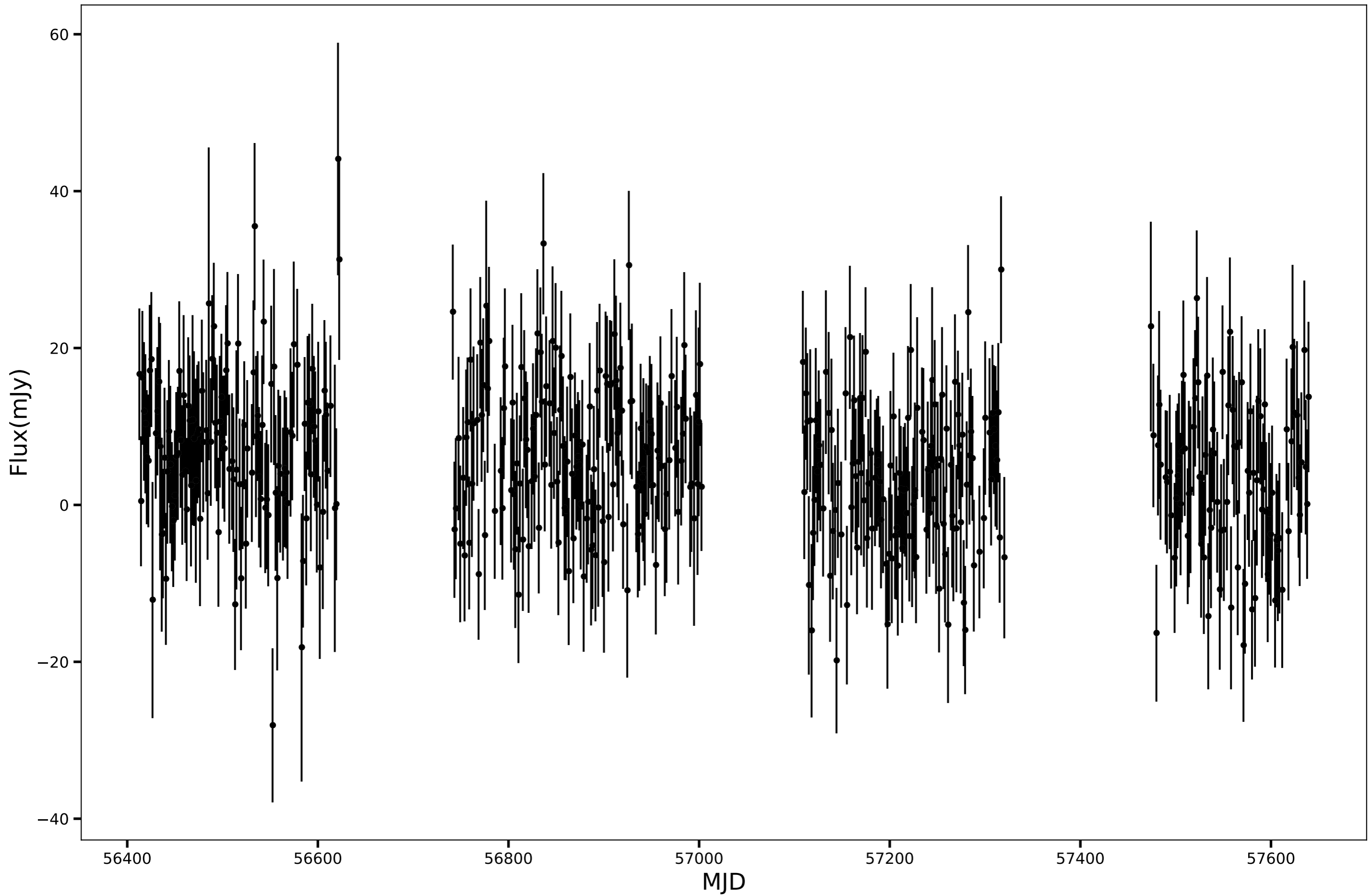
SPT-SJ224706-5408.9, RA=341.7772d, DEC=-54.1487d, mean_flux=5.26 (mJy)
