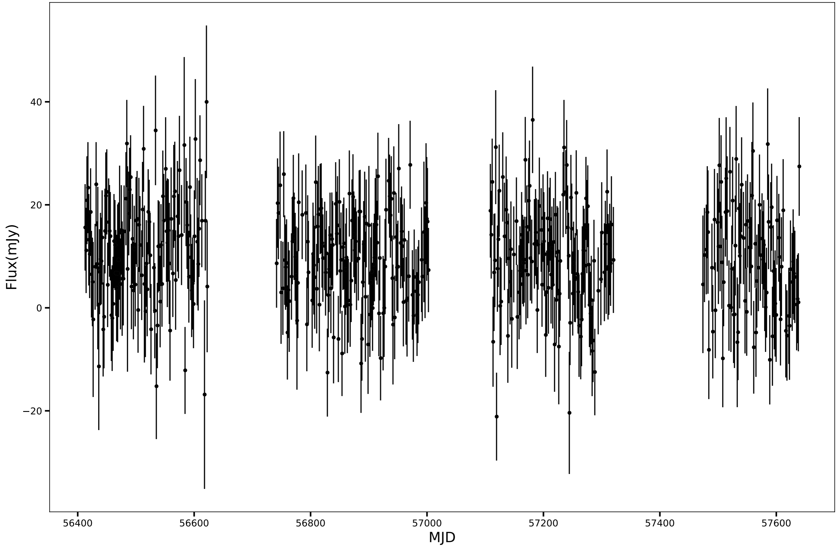
SPT-SJ222702-5233.5, RA=336.7588d, DEC=-52.5585d, mean_flux=9.87 (mJy)
