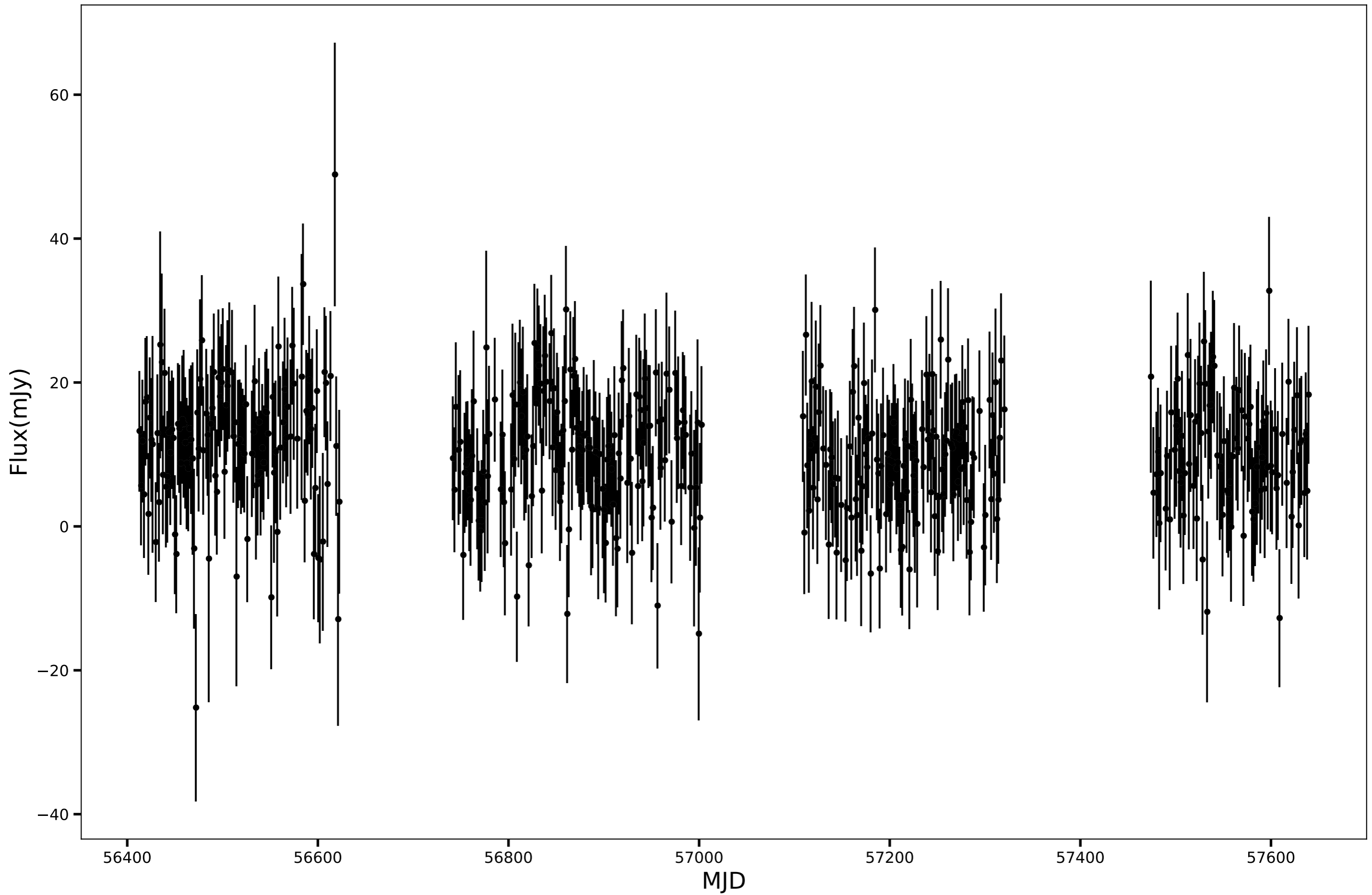
SPT-SJ222658-6237.8, RA=336.7419d, DEC=-62.6306d, mean_flux=10.33 (mJy)
