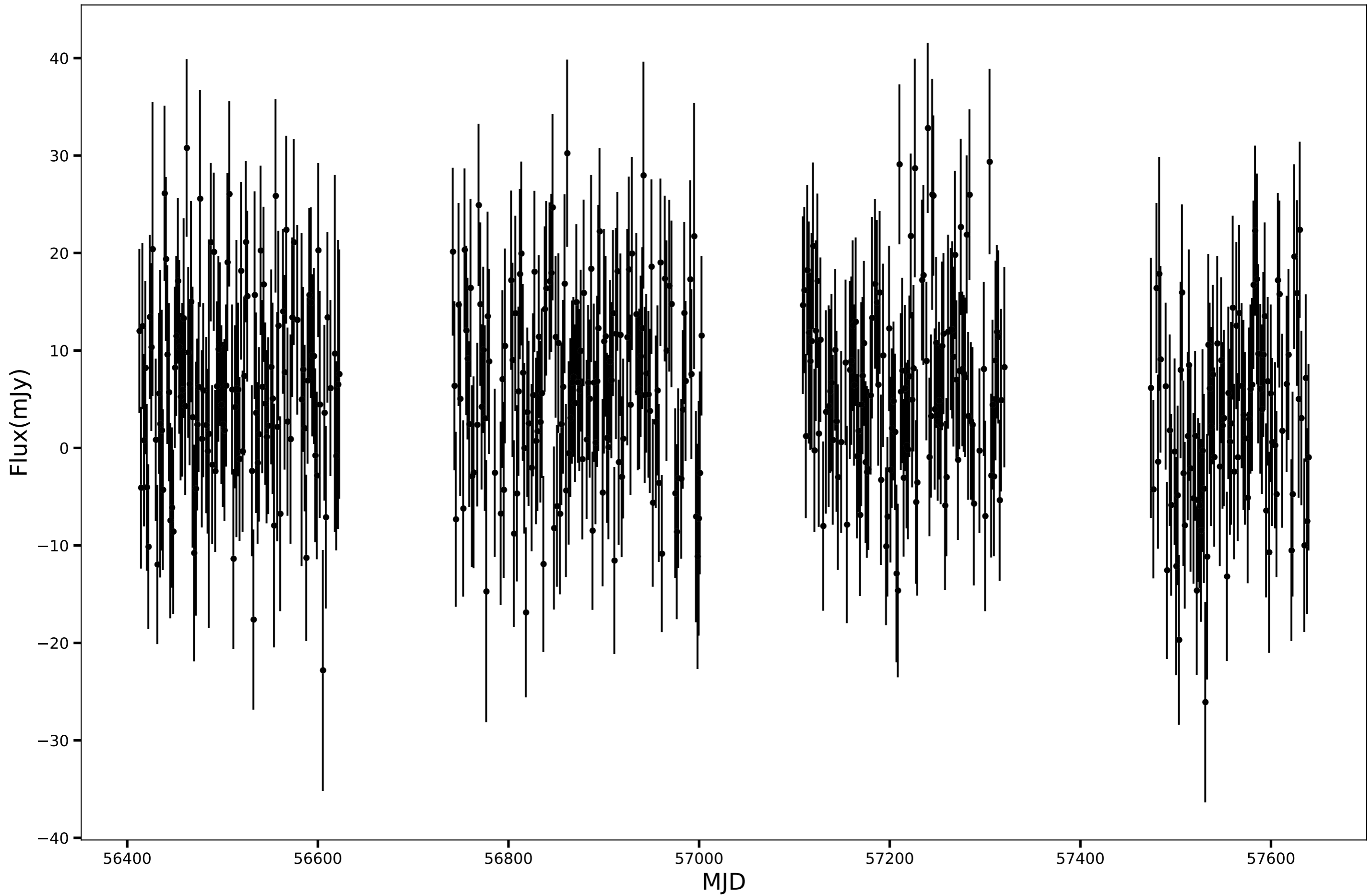
SPT-SJ222330-5017.1, RA=335.8761d, DEC=-50.2853d, mean_flux=5.73 (mJy)
