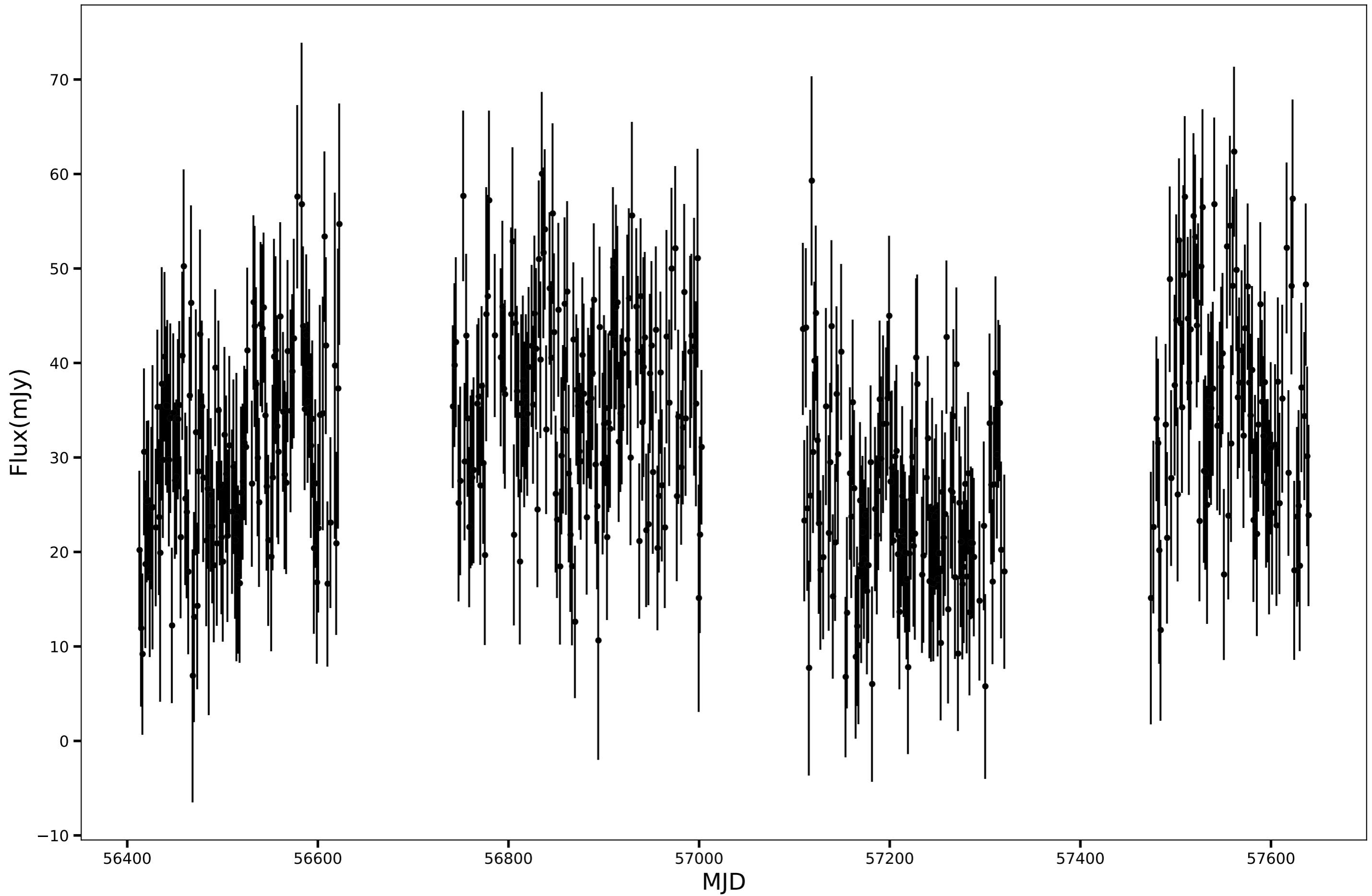
SPT-SJ221642-5637.5, RA=334.1768d, DEC=-56.6259d, mean_flux=31.89 (mJy)
