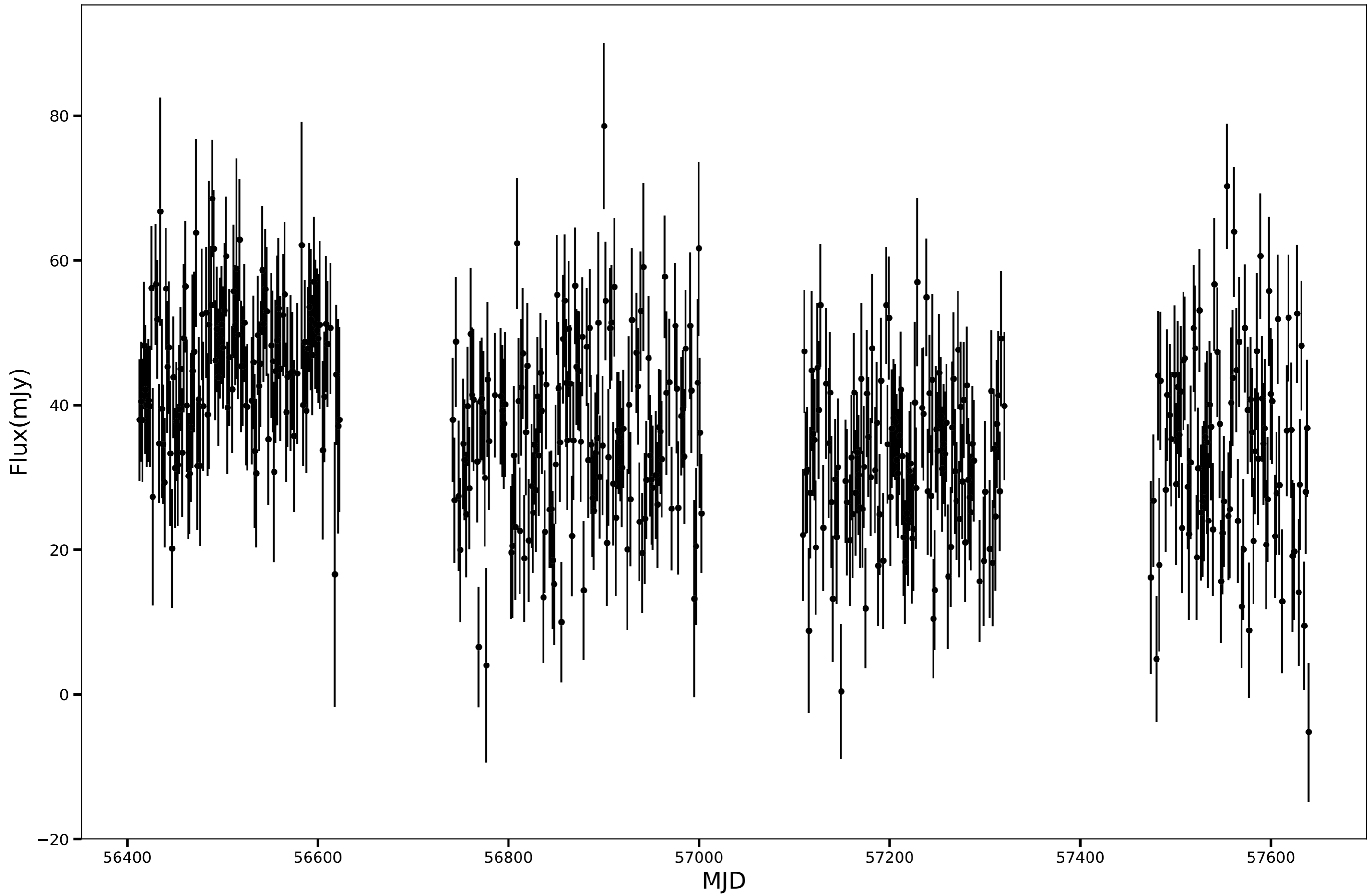
SPT-SJ220253-5635.7, RA=330.7210d, DEC=-56.5953d, mean_flux=36.93 (mJy)
