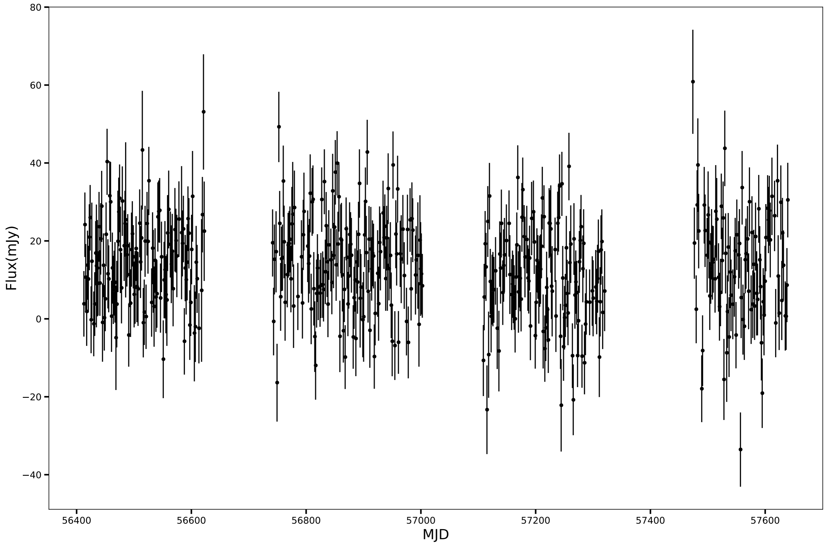
SPT-SJ220014-5410.9, RA=330.0608d, DEC=-54.1833d, mean_flux=13.23 (mJy)
