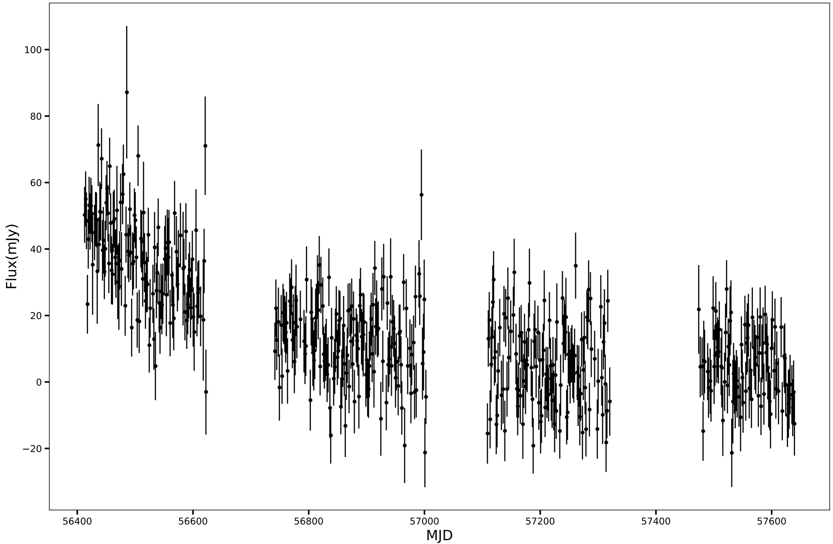
SPT-SJ215648-6331.0, RA=329.209d, DEC=-63.5179d, mean_flux=15.26 (mJy)
