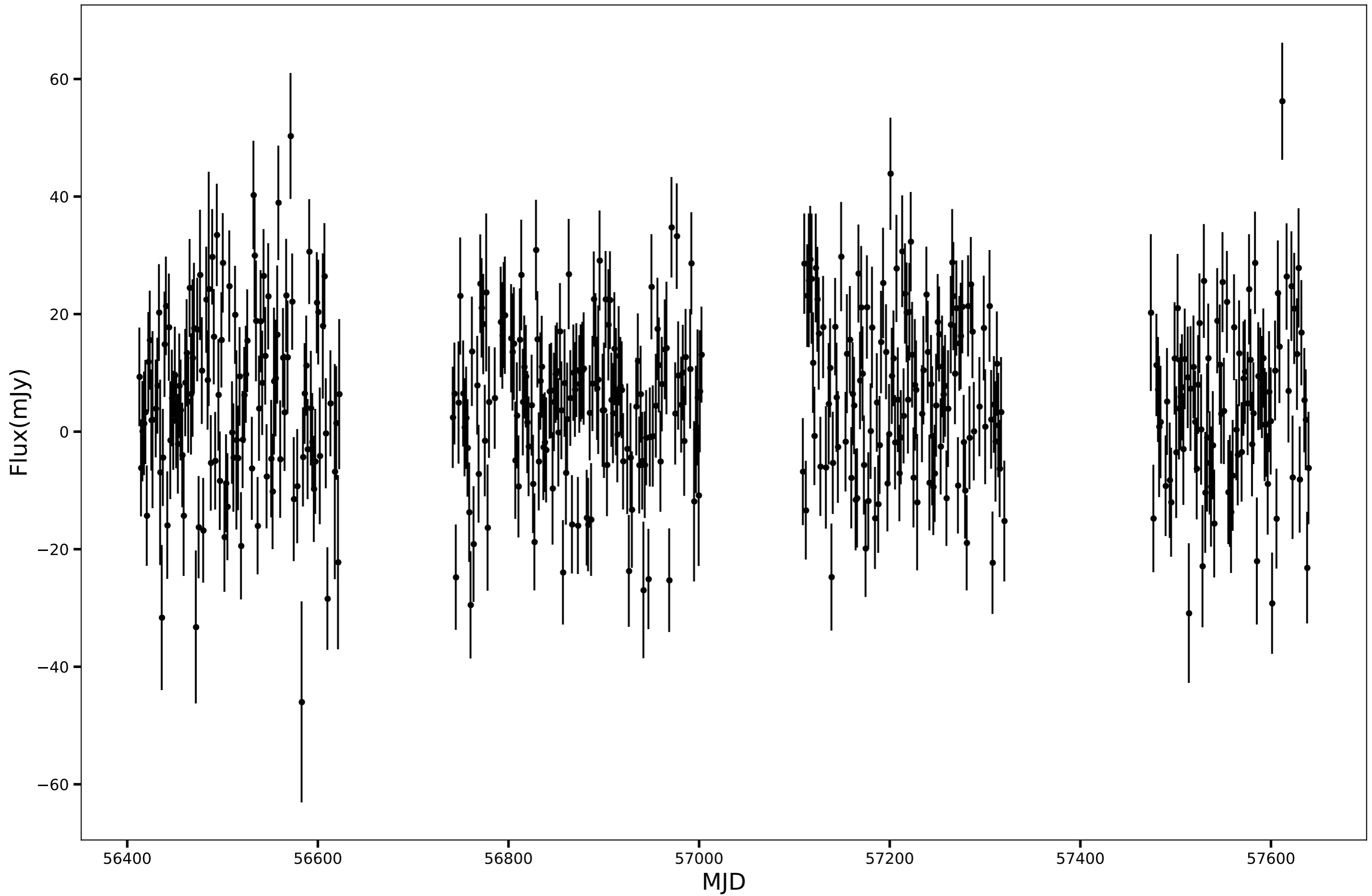
SPT-SJ215608-5017.7, RA=329.0339d, DEC=-50.2955d, mean_flux=5.44 (mJy)
