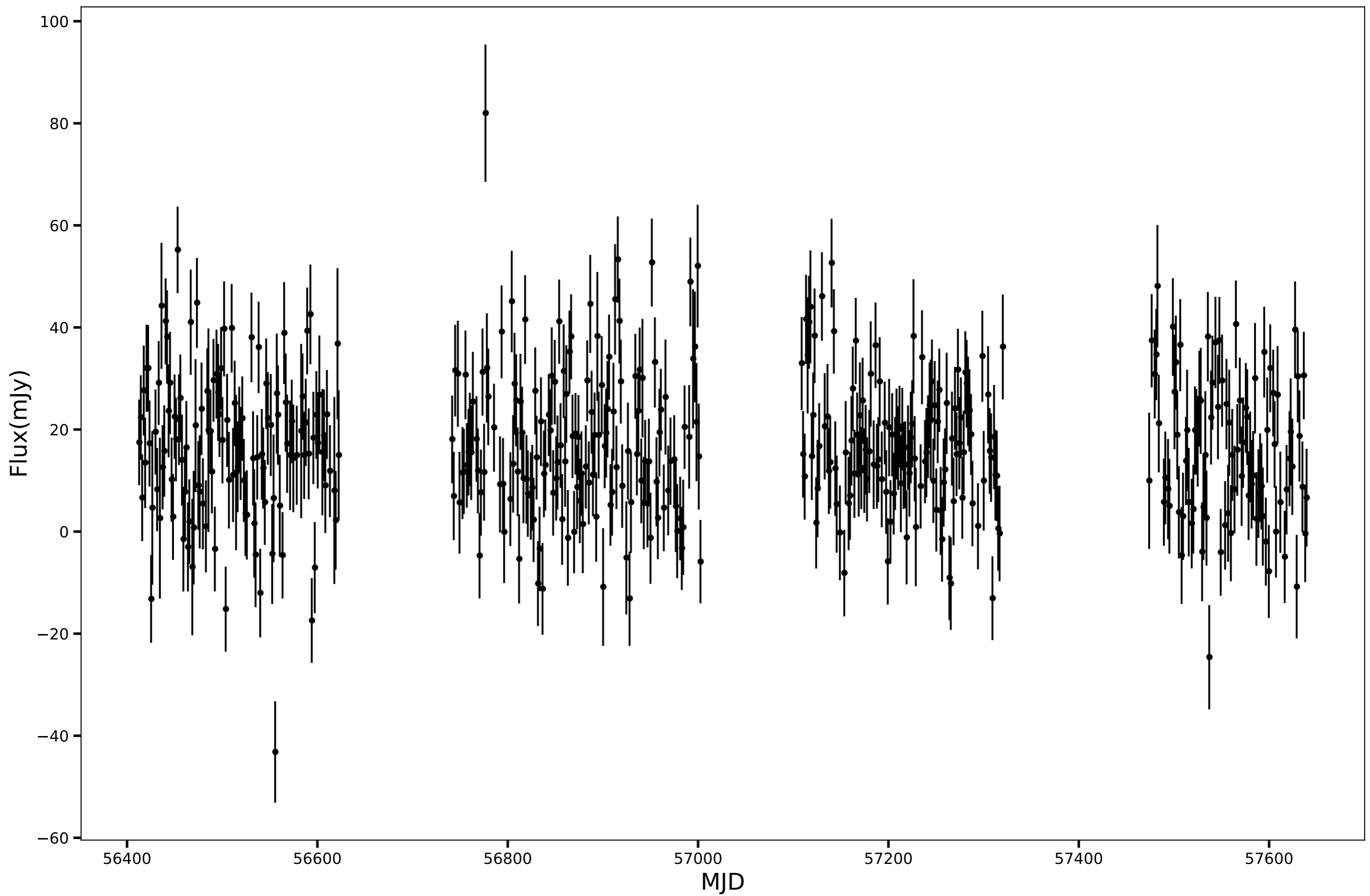
SPT-SJ215459-5930.4, RA=328.7484d, DEC=-59.5080d, mean_flux=16.85 (mJy)
