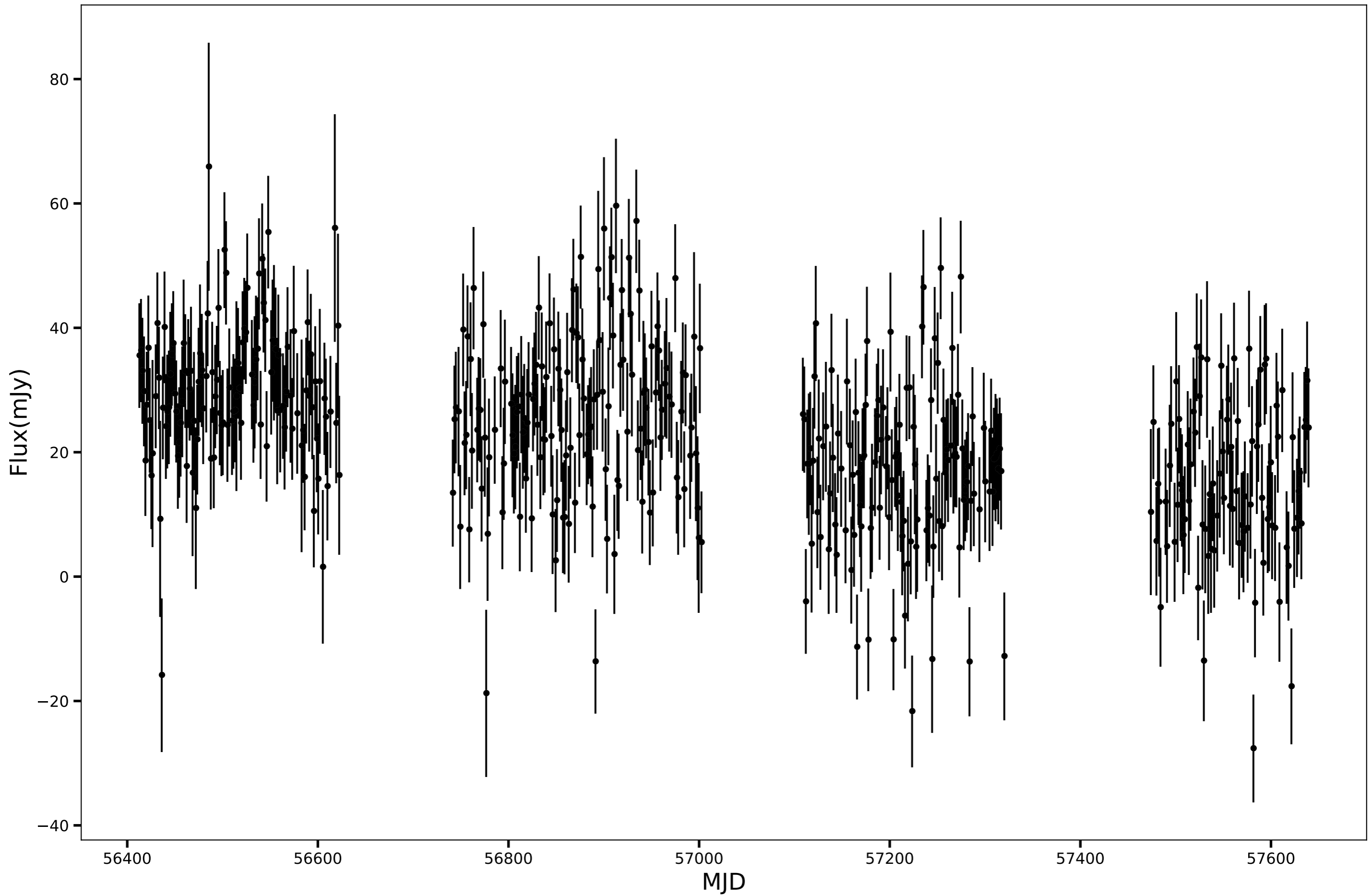
SPT-SJ015912-5308.7, RA=29.8039d, DEC=-53.1465d, mean_flux=22.58 (mJy)
