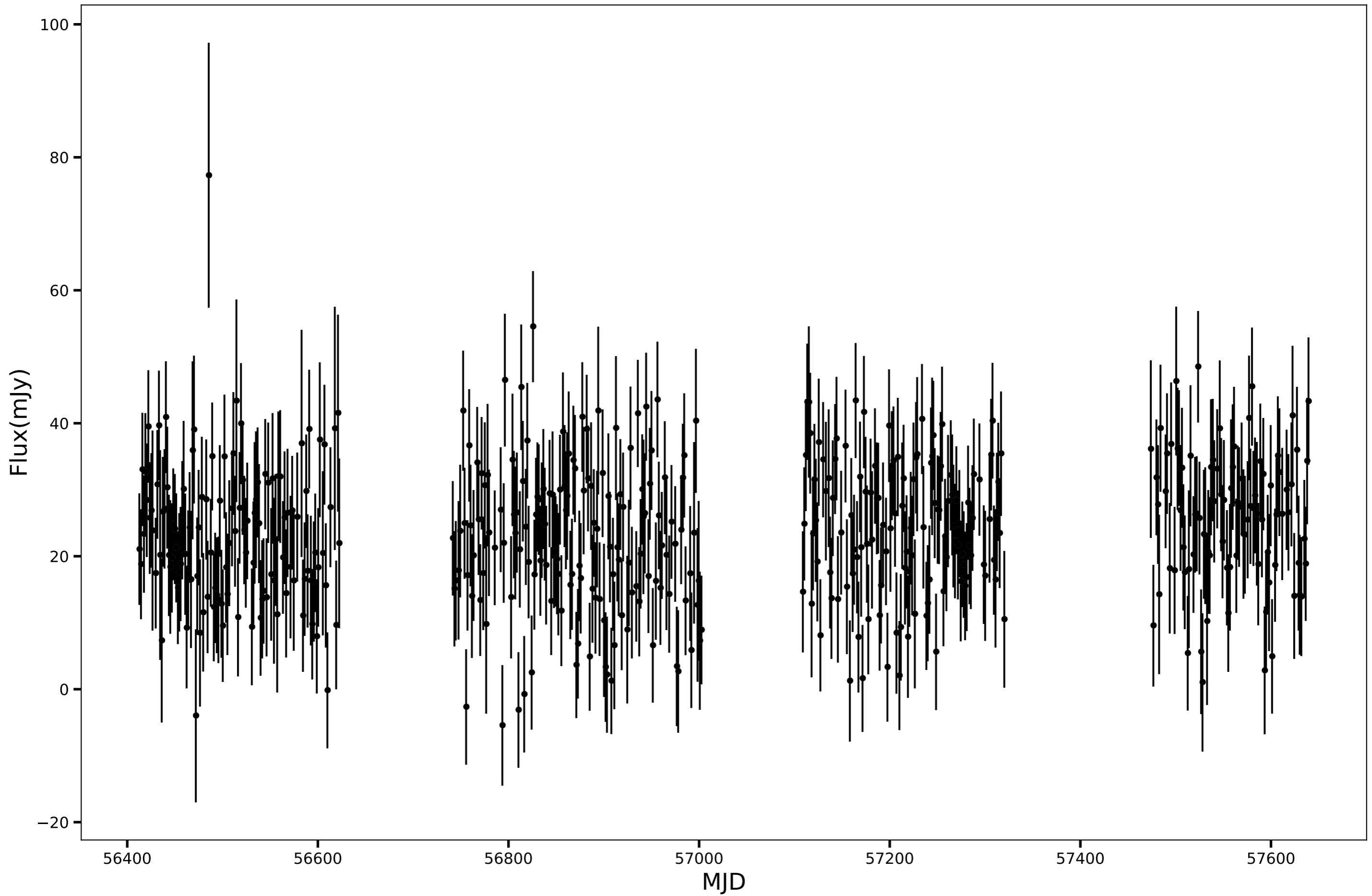
SPT-SJ015853-6334.8, RA=29.7244d, DEC=-63.5801d, mean_flux=23.76 (mJy)
