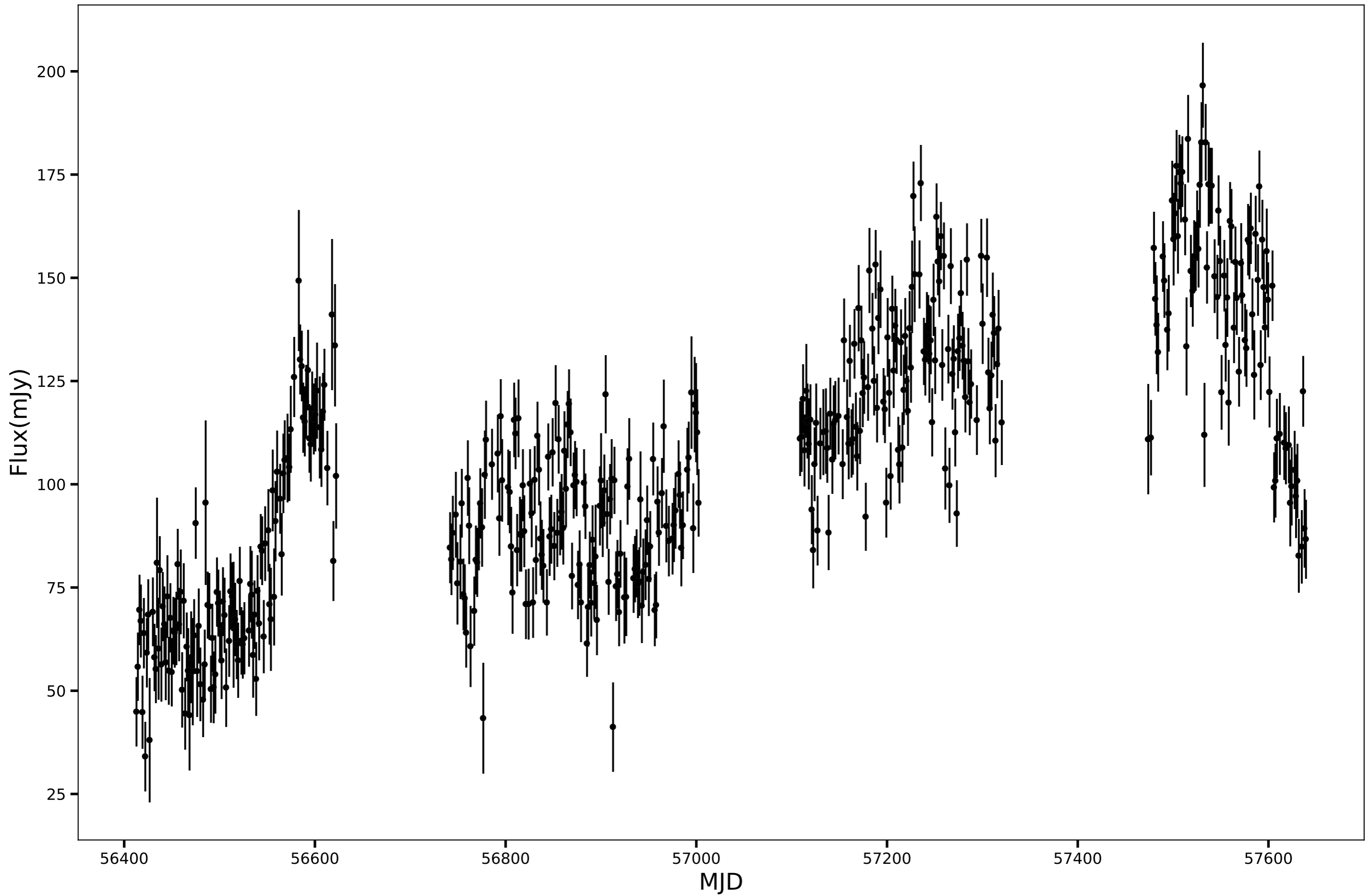
SPT-SJ015826-5810.9, RA=29.6114d, DEC=-58.1823d, mean_flux=105.85 (mJy)
