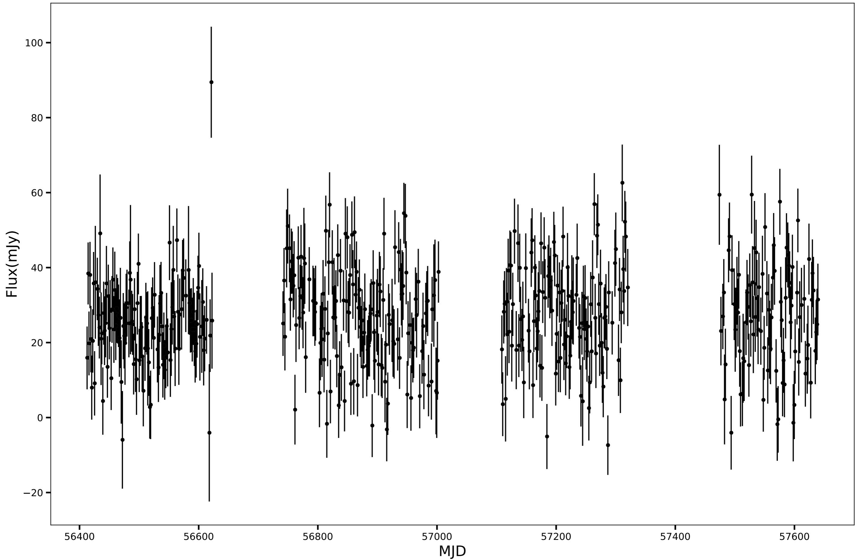
SPT-SJ015816-5004.3, RA=29.5677d, DEC=-50.0732d, mean_flux=26.64 (mJy)
