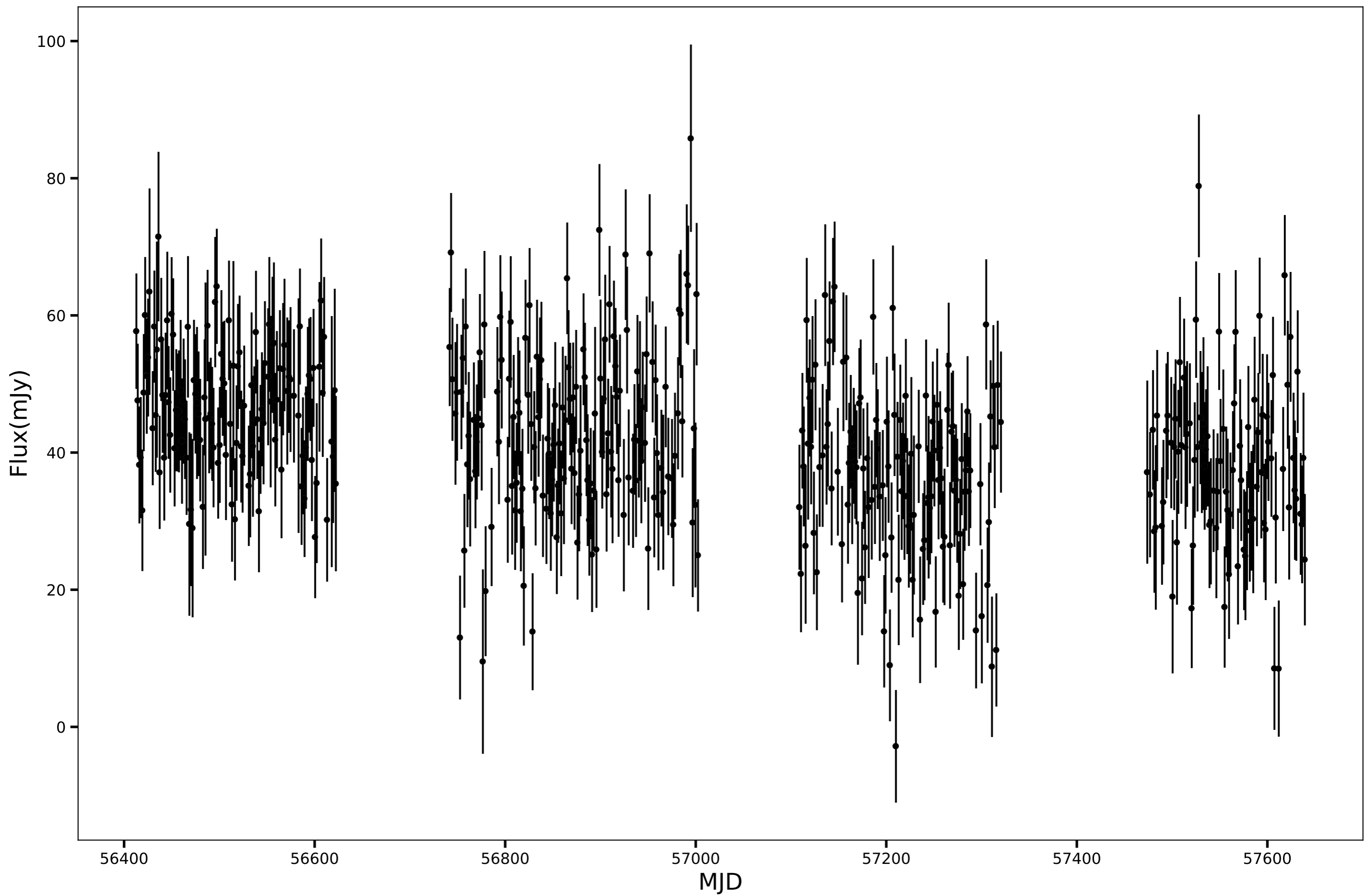
SPT-SJ015650-5439.7, RA=29.2110d, DEC=-54.6620d, mean_flux=41.42 (mJy)
