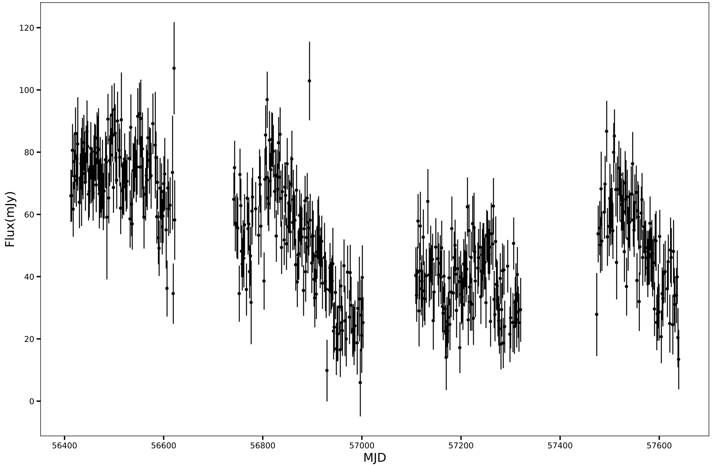
SPT-SJ015509-6425.5, RA=28.7913d, DEC=-64.4250d, mean_flux=53.34 (mJy)
