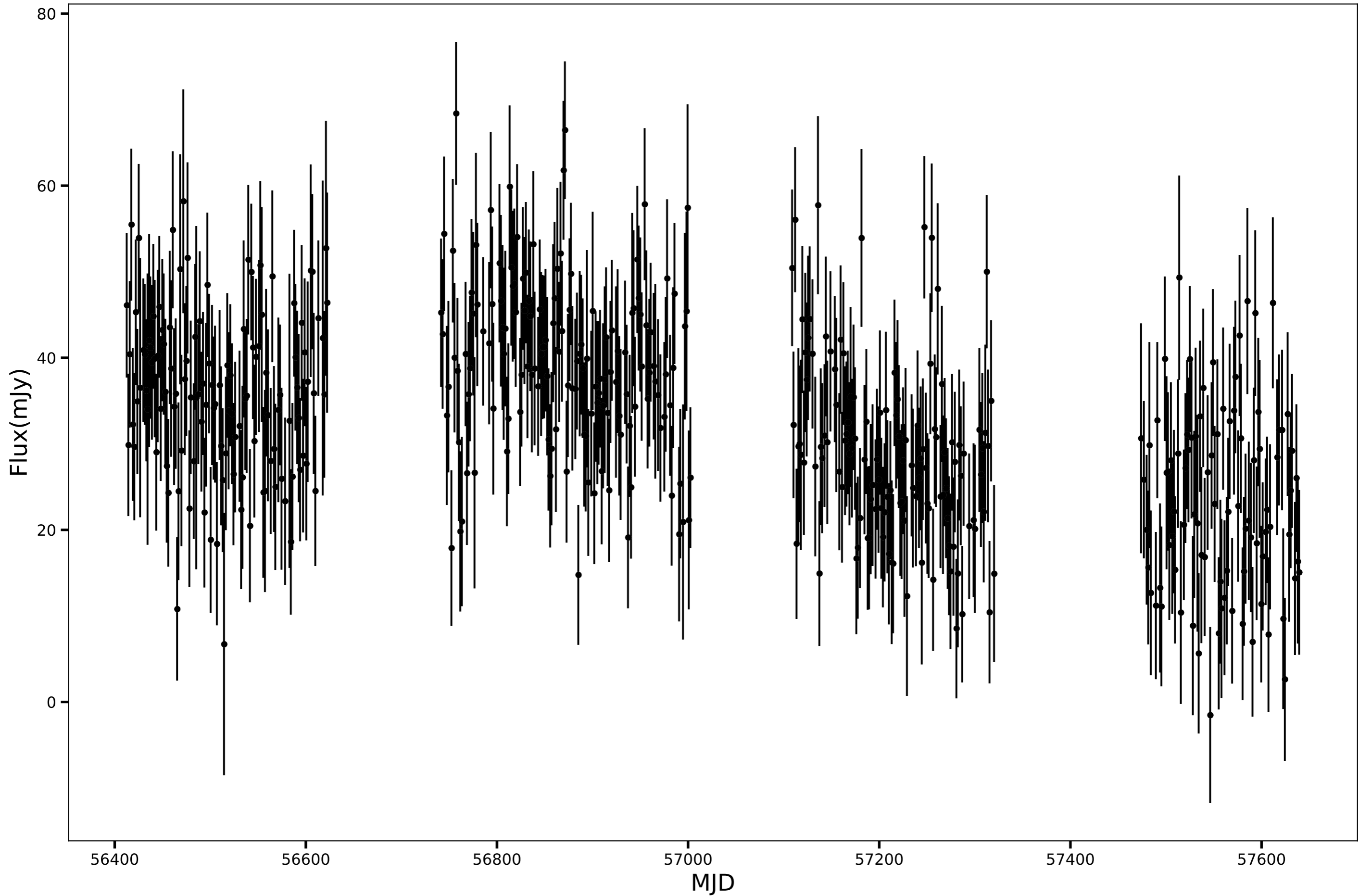
SPT-SJ015357-5406.8, RA=28.4912d, DEC=-54.1144d, mean_flux=32.83 (mJy)
