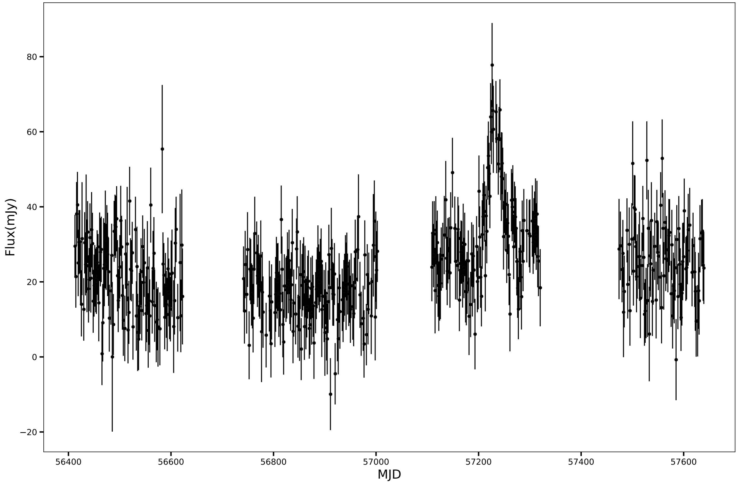
SPT-SJ015050-6044.2, RA=27.7096d, DEC=-60.7368d, mean_flux=23.72 (mJy)
