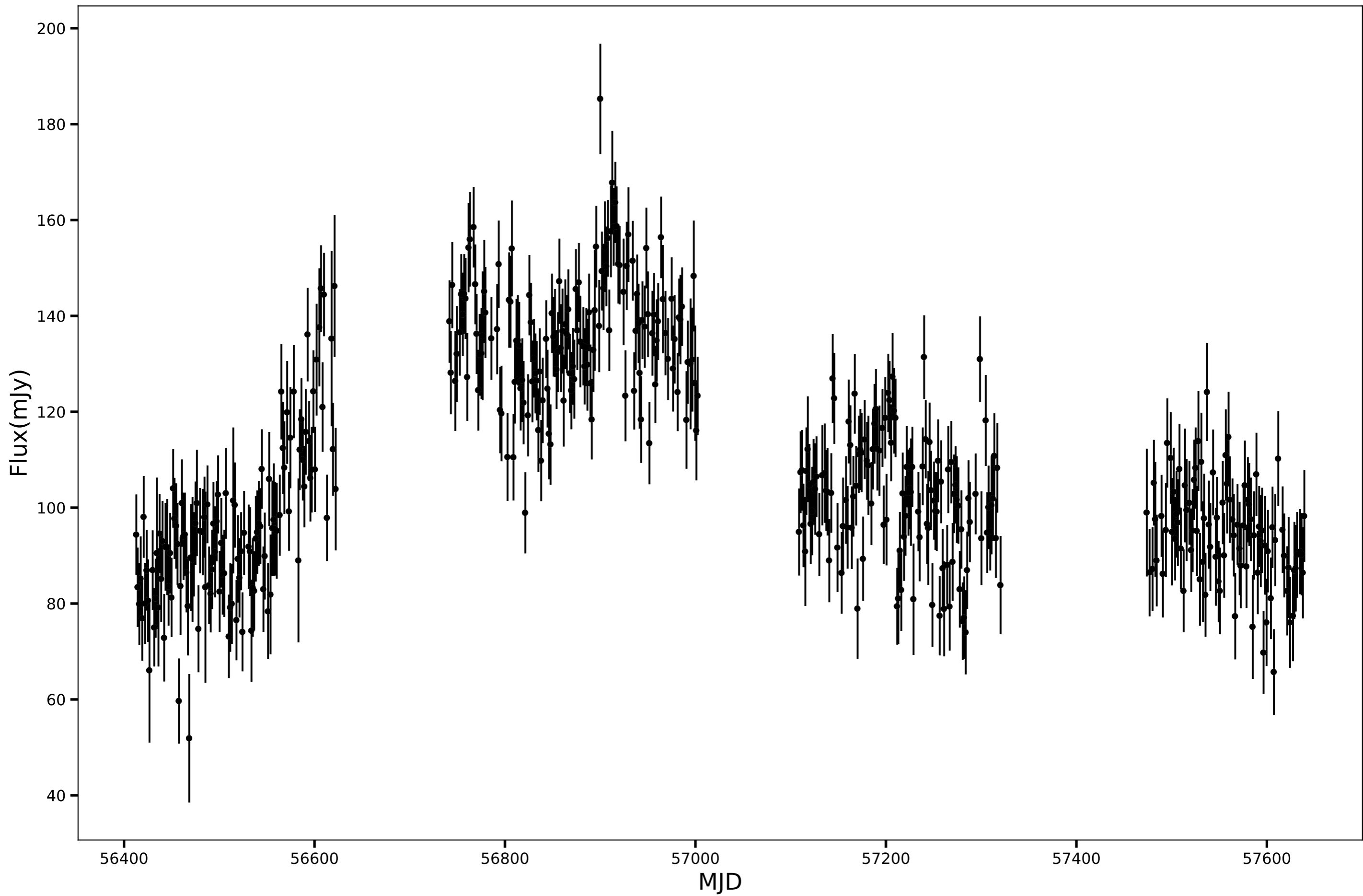
SPT-SJ014648-5202.5, RA=26.7001d, DEC=-52.0423d, mean_flux=109.23 (mJy)
