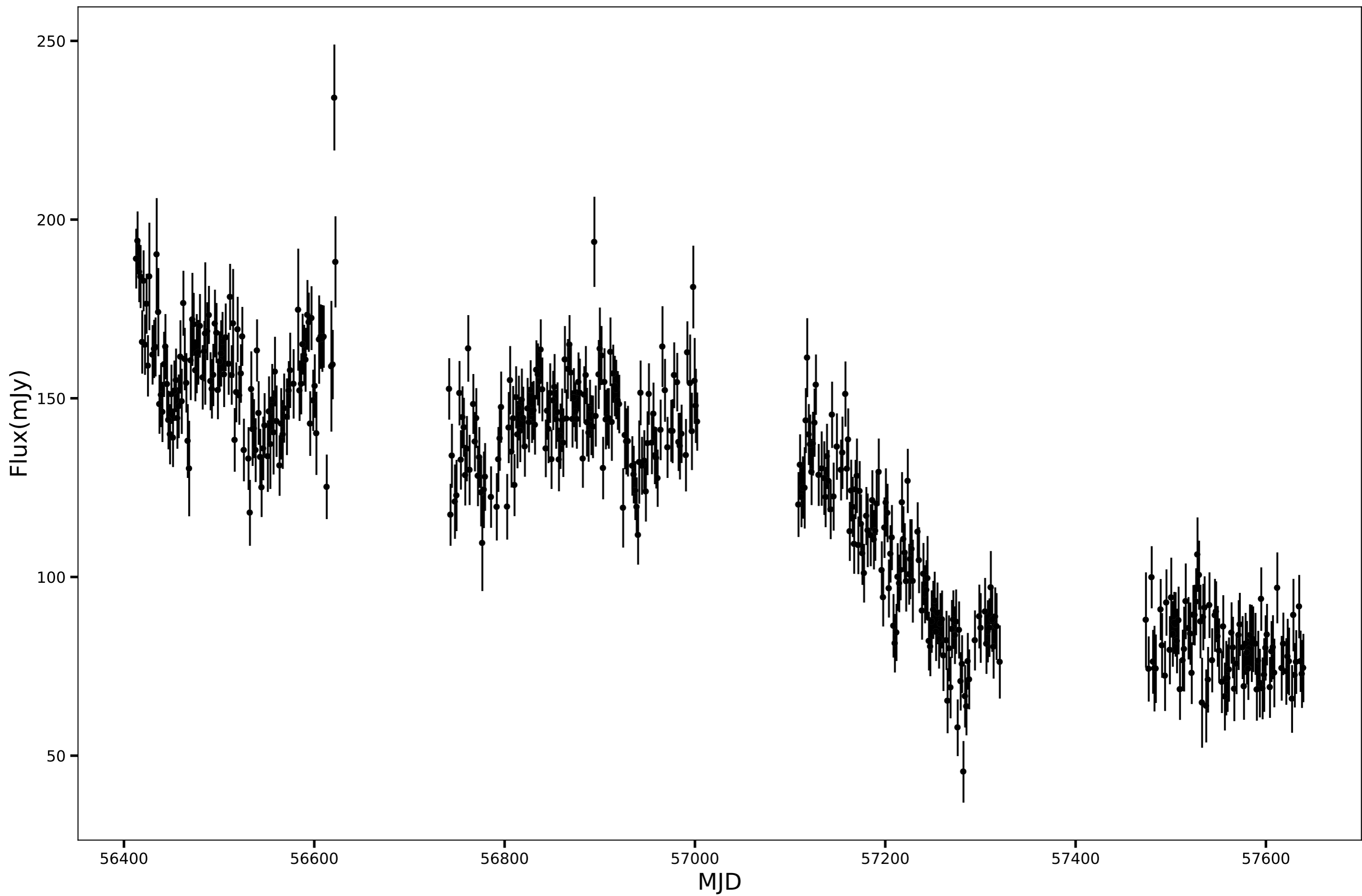
SPT-SJ014415-6421.8, RA=26.0657d, DEC=-64.3648d, mean_flux=125.24 (mJy)
