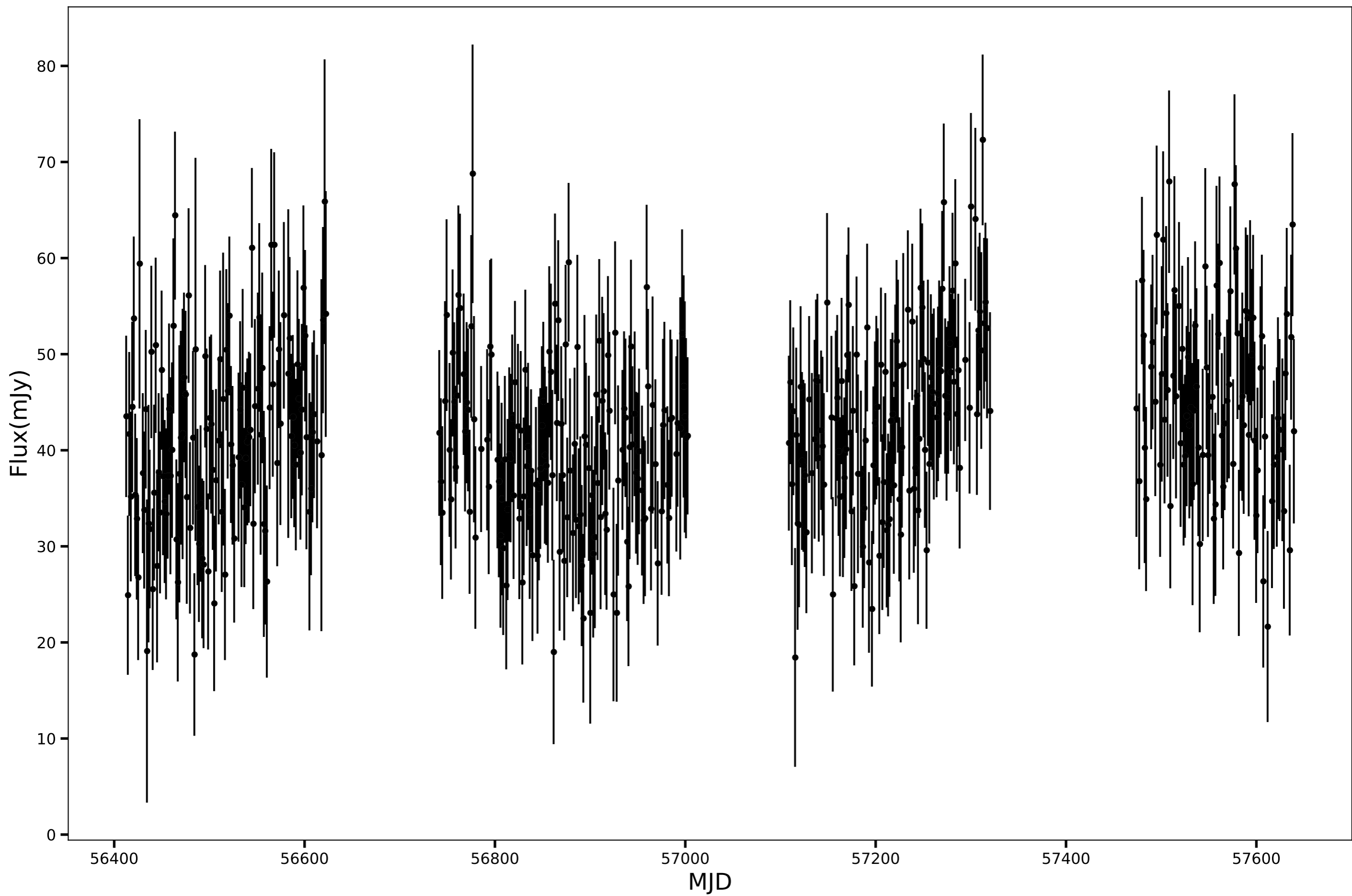
SPT-SJ014257-6044.9, RA=25.7376d, DEC=-60.7498d, mean_flux=42.12 (mJy)
