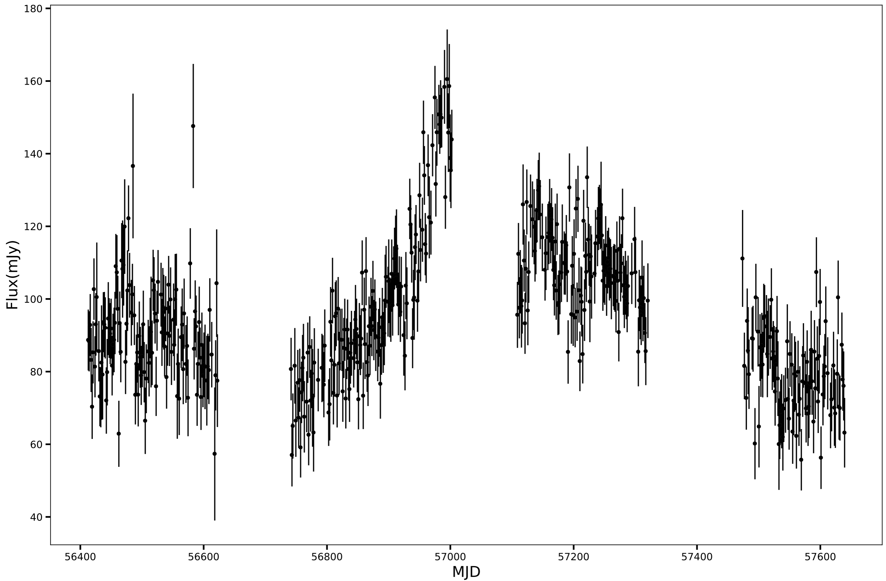
SPT-SJ014225-5729.8, RA=25.6081d, DEC=-57.4982d, mean_flux=95.11 (mJy)
