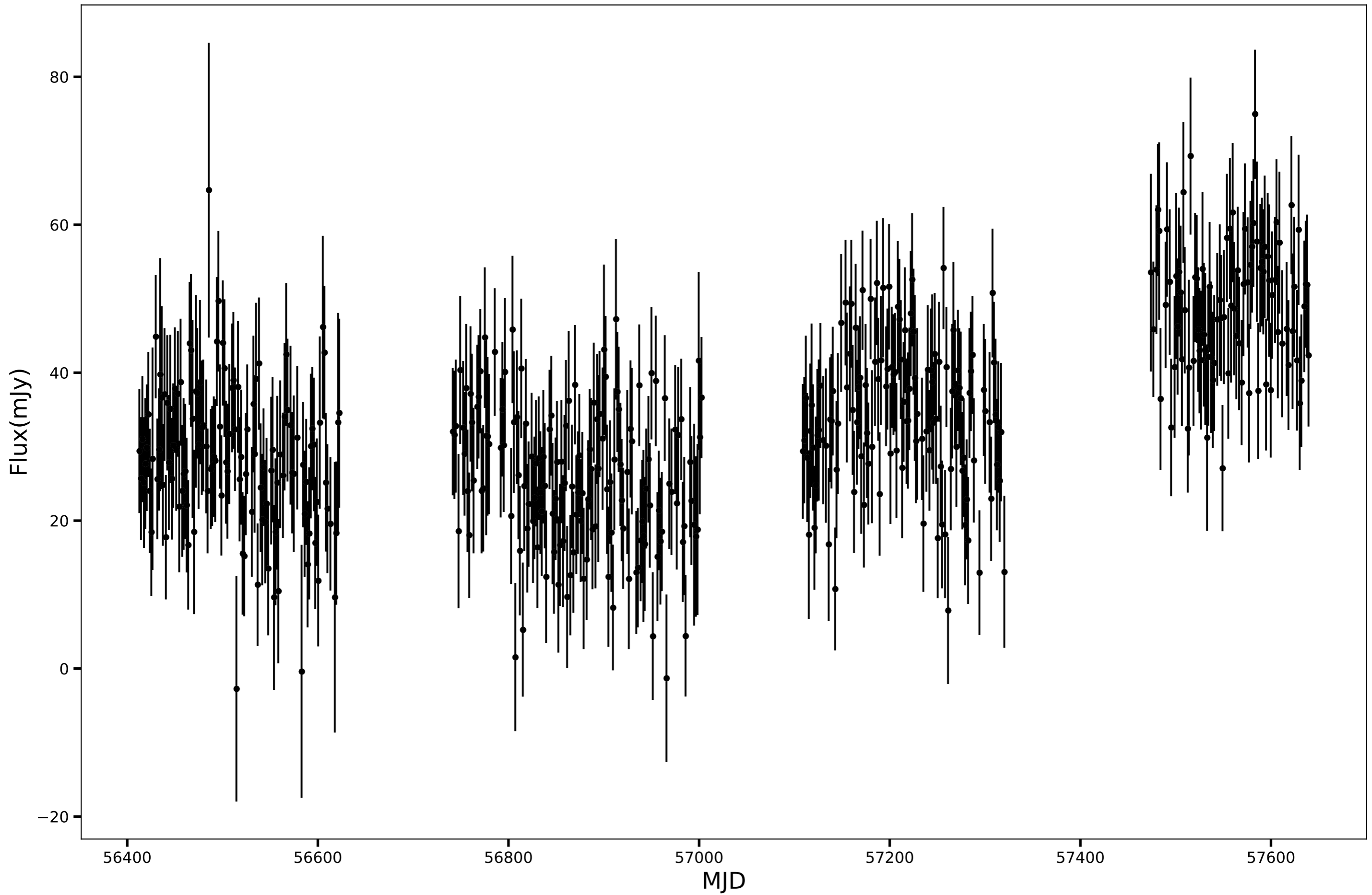
SPT-SJ014142-5650.6, RA=25.4274d, DEC=-56.8442d, mean_flux=33.04 (mJy)
