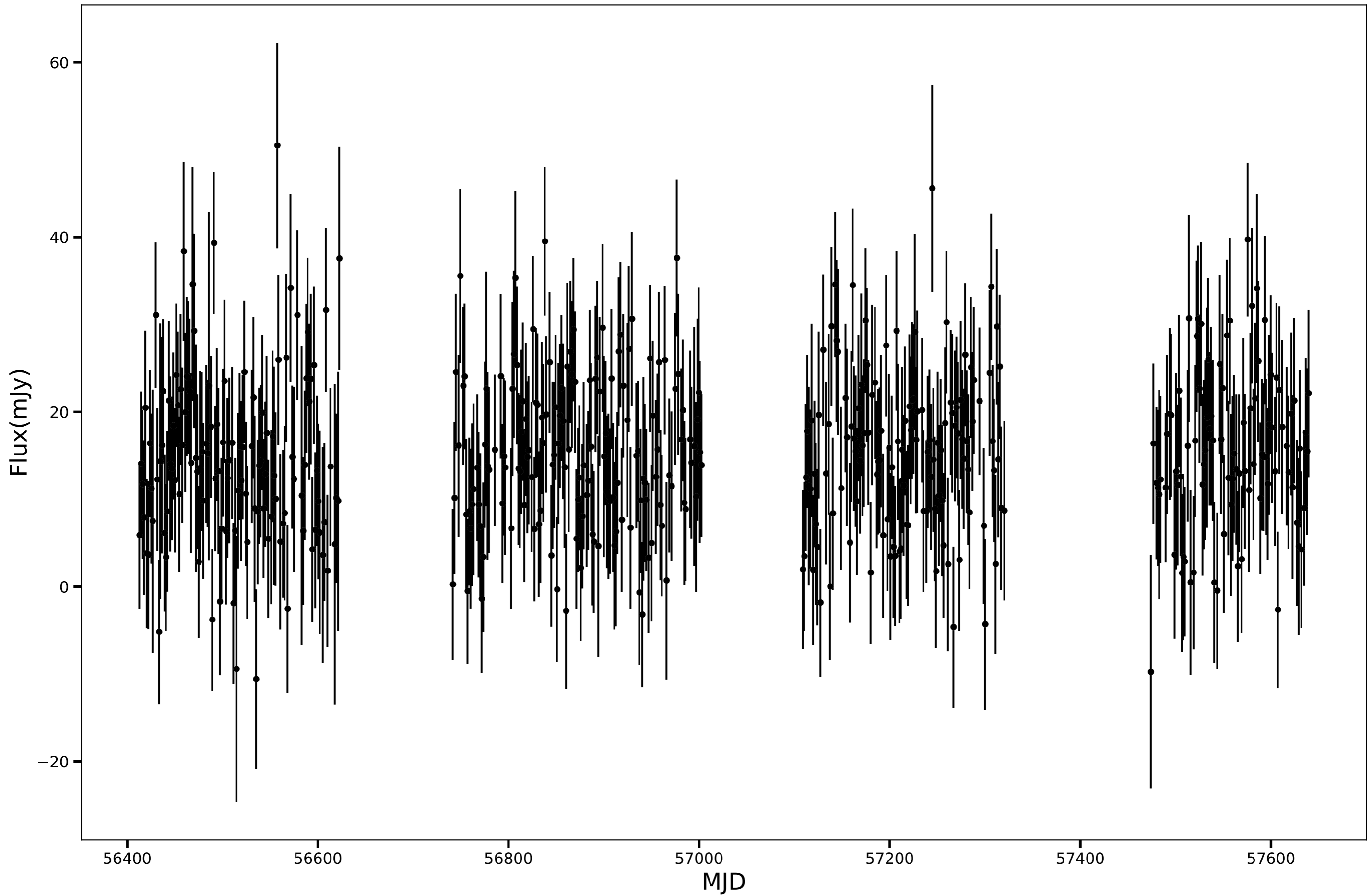
SPT-SJ014132-5427.8, RA=25.3836d, DEC=-54.4636d, mean_flux=15.14 (mJy)
