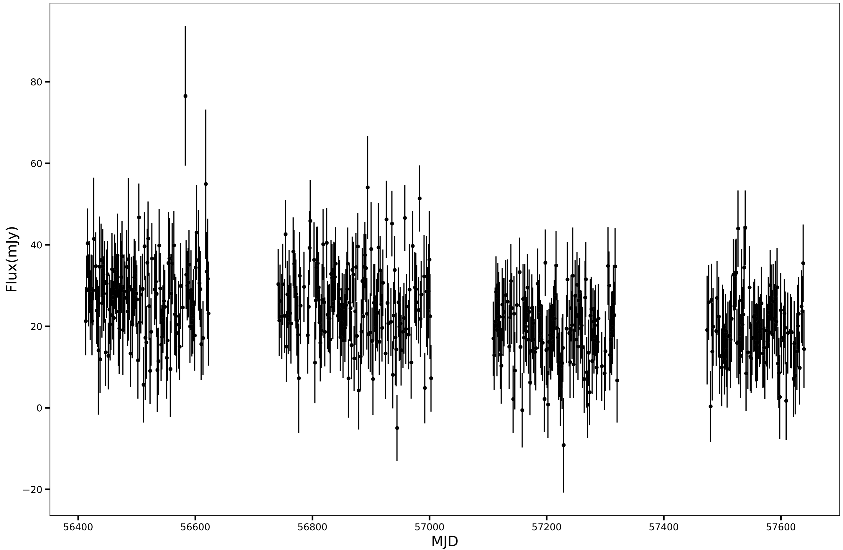
SPT-SJ013408-5526.3, RA=23.5375d, DEC=-55.4396d, mean_flux=23.04 (mJy)
