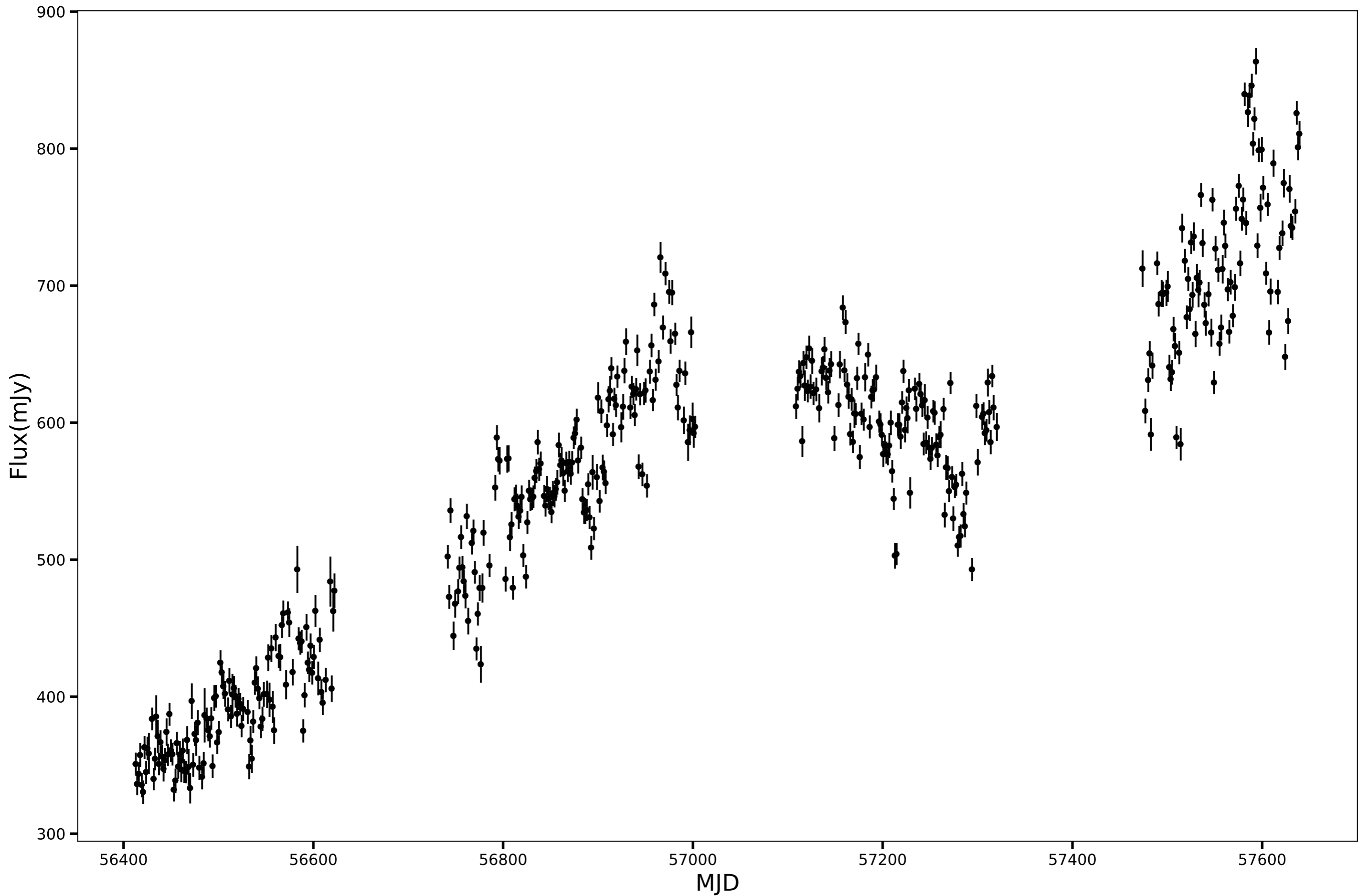
SPT-SJ013305-5200.1, RA=23.2711d, DEC=-52.0018d, mean_flux=558.46 (mJy)
