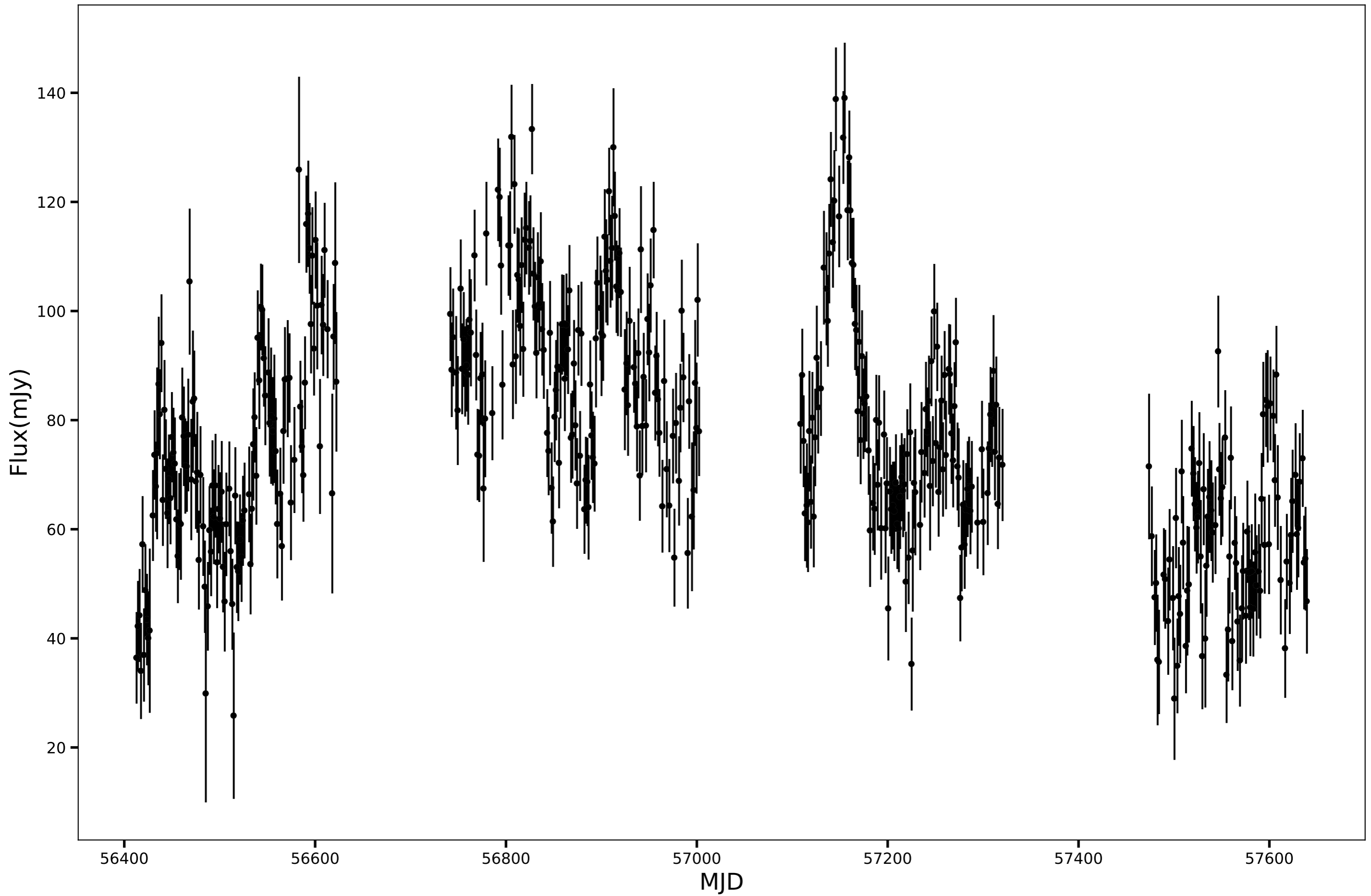
SPT-SJ012820-5649.6, RA=22.0855d, DEC=-56.8276d, mean_flux=76.90 (mJy)
