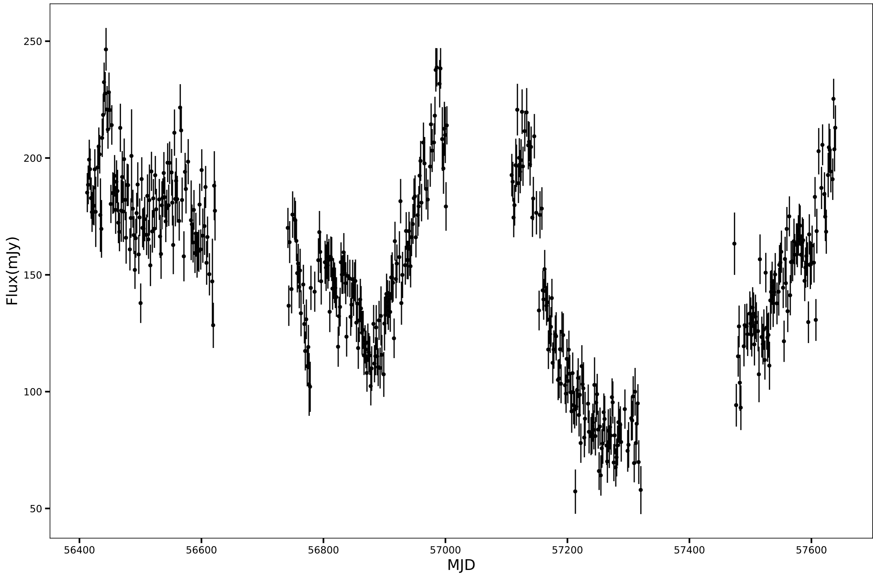
SPT-SJ012456-5113.1, RA=21.2366d, DEC=-51.2199d, mean_flux=150.96 (mJy)
