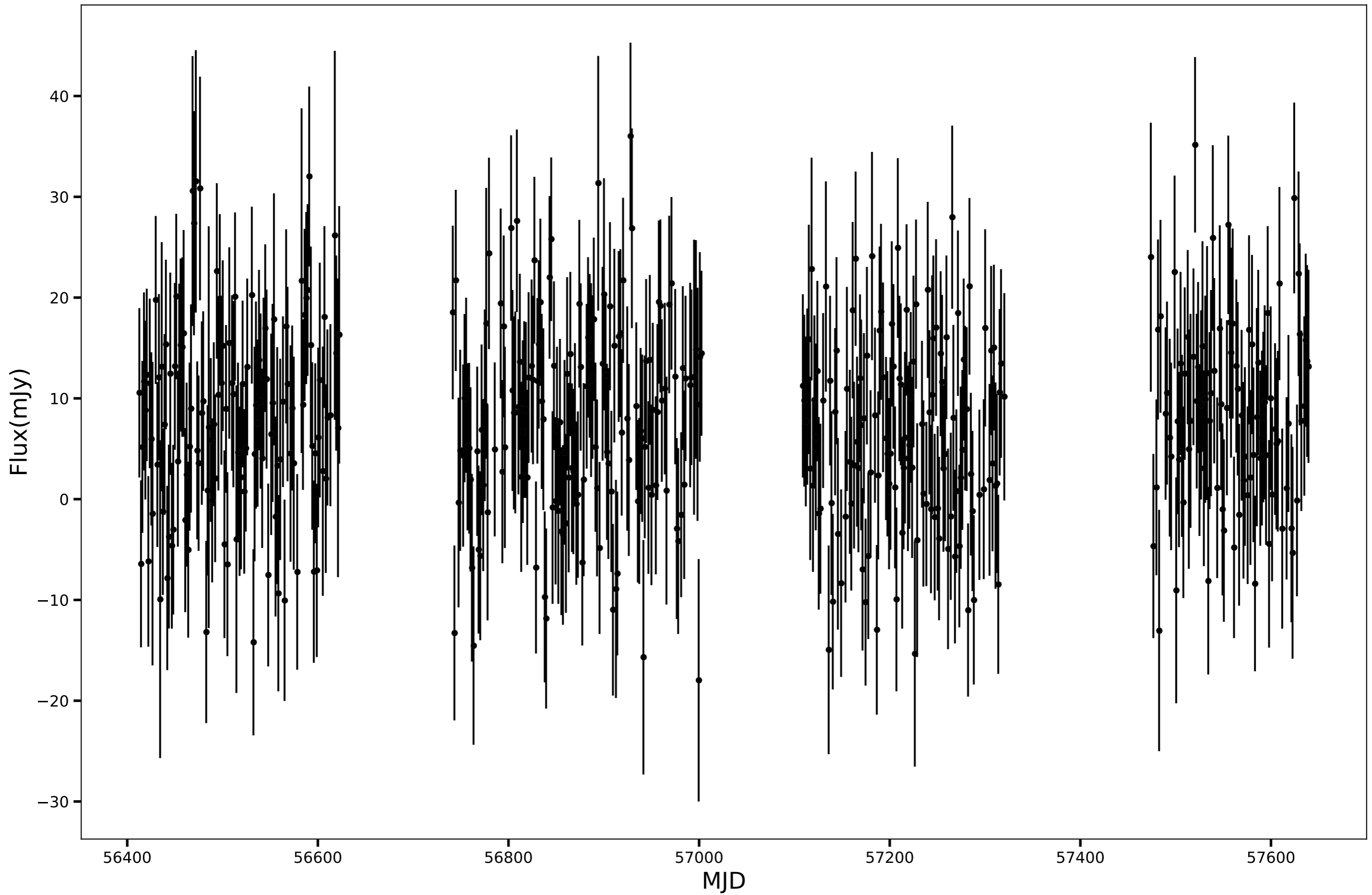
SPT-SJ012110-5602.6, RA=20.2927d, DEC=-56.0443d, mean_flux=7.57 (mJy)
