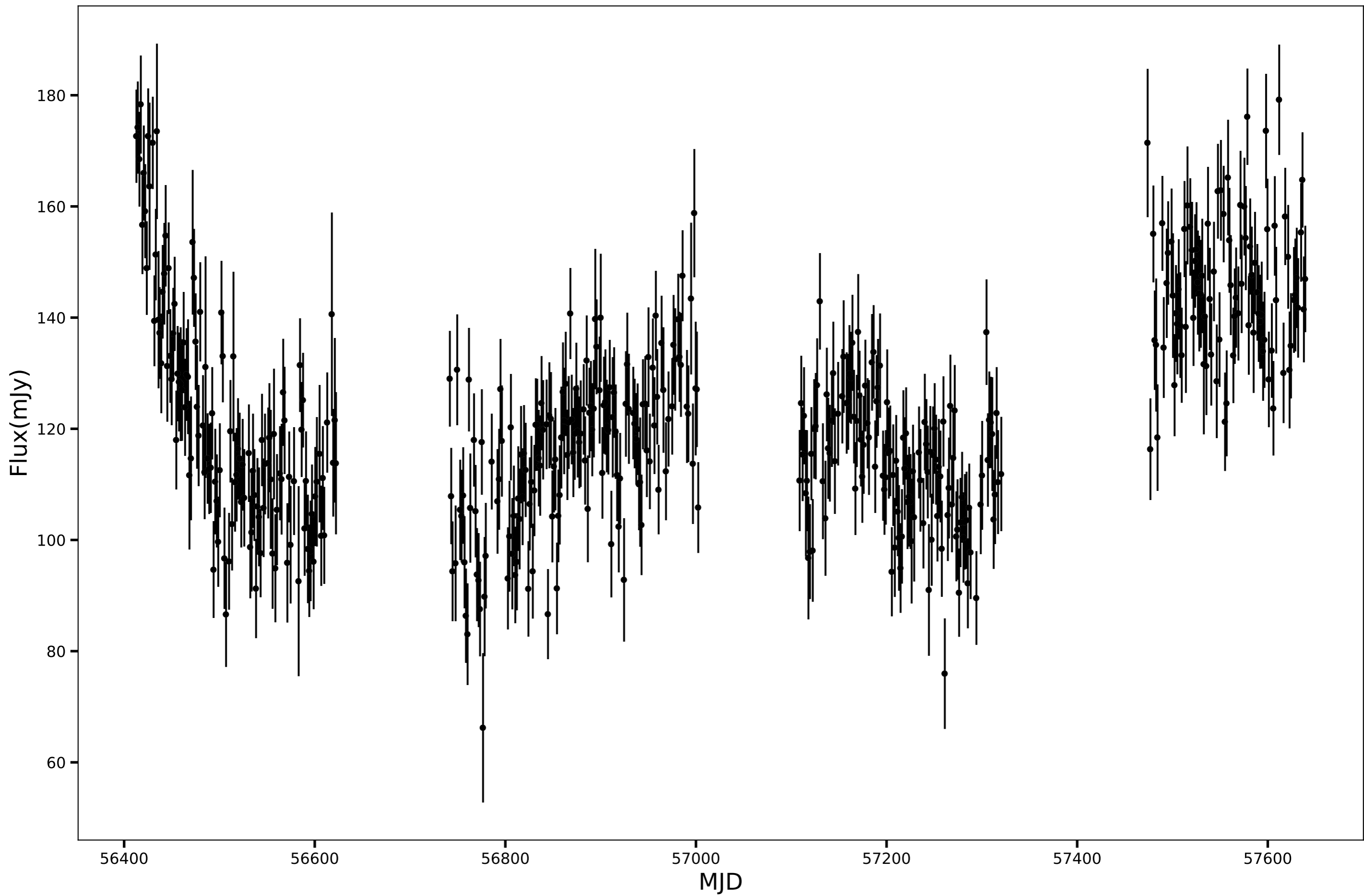
SPT-SJ011950-5357.2, RA=19.9614d, DEC=-53.9546d, mean_flux=122.50 (mJy)
