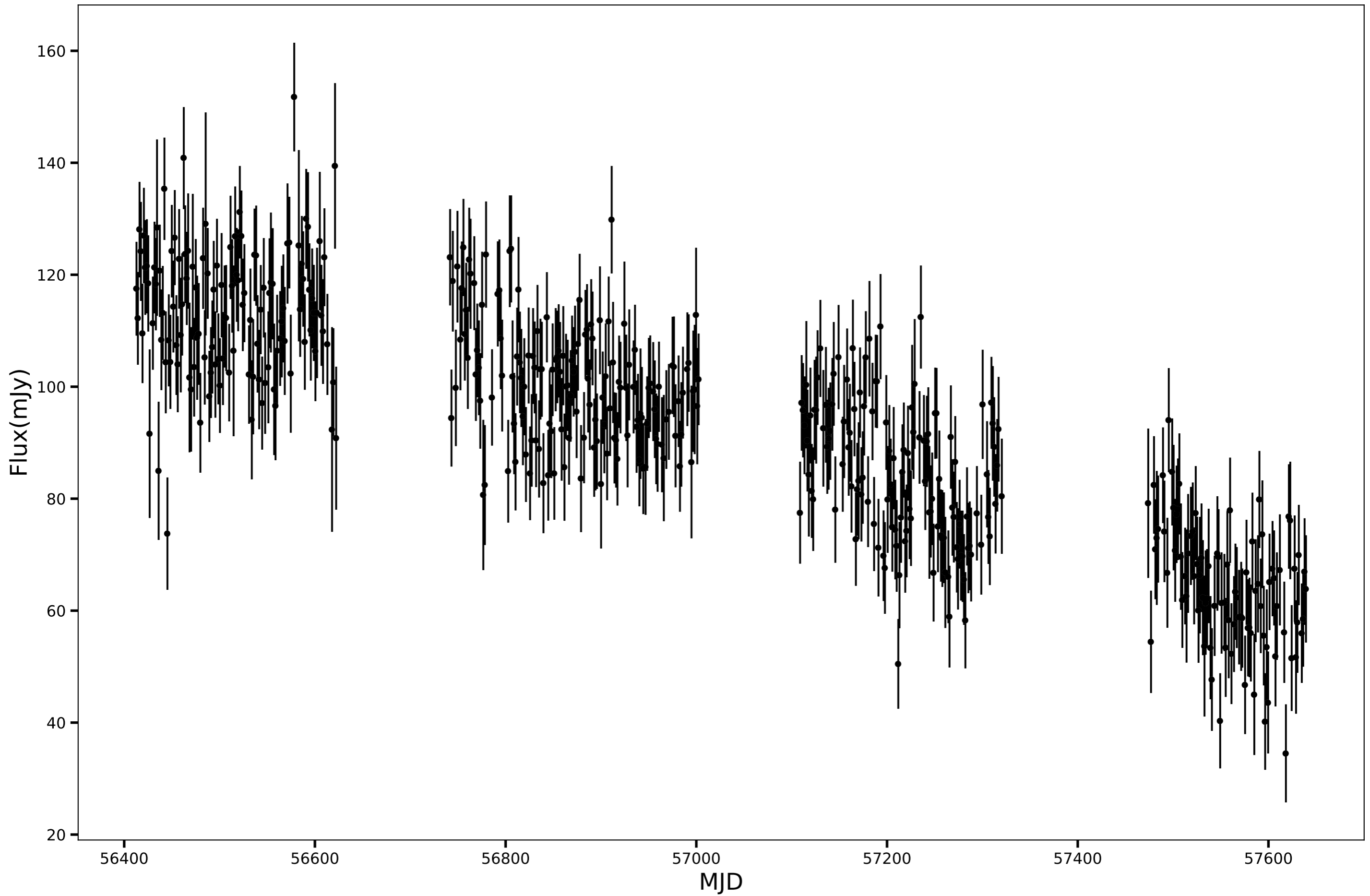
SPT-SJ011016-6316.0, RA=17.5688d, DEC=-63.2669d, mean_flux=92.97 (mJy)
