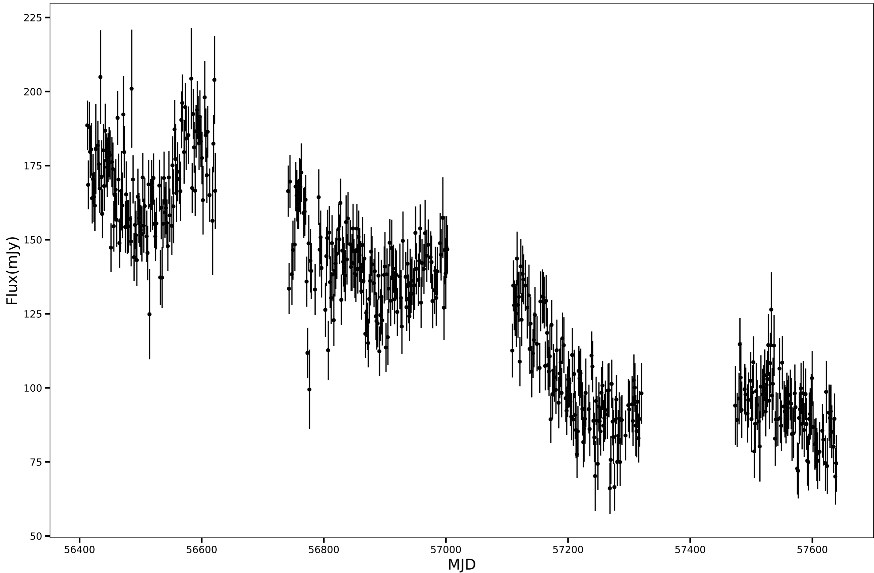
SPT-SJ010915-6049.8, RA=17.3143d, DEC=-60.8301d, mean_flux=128.94 (mJy)
