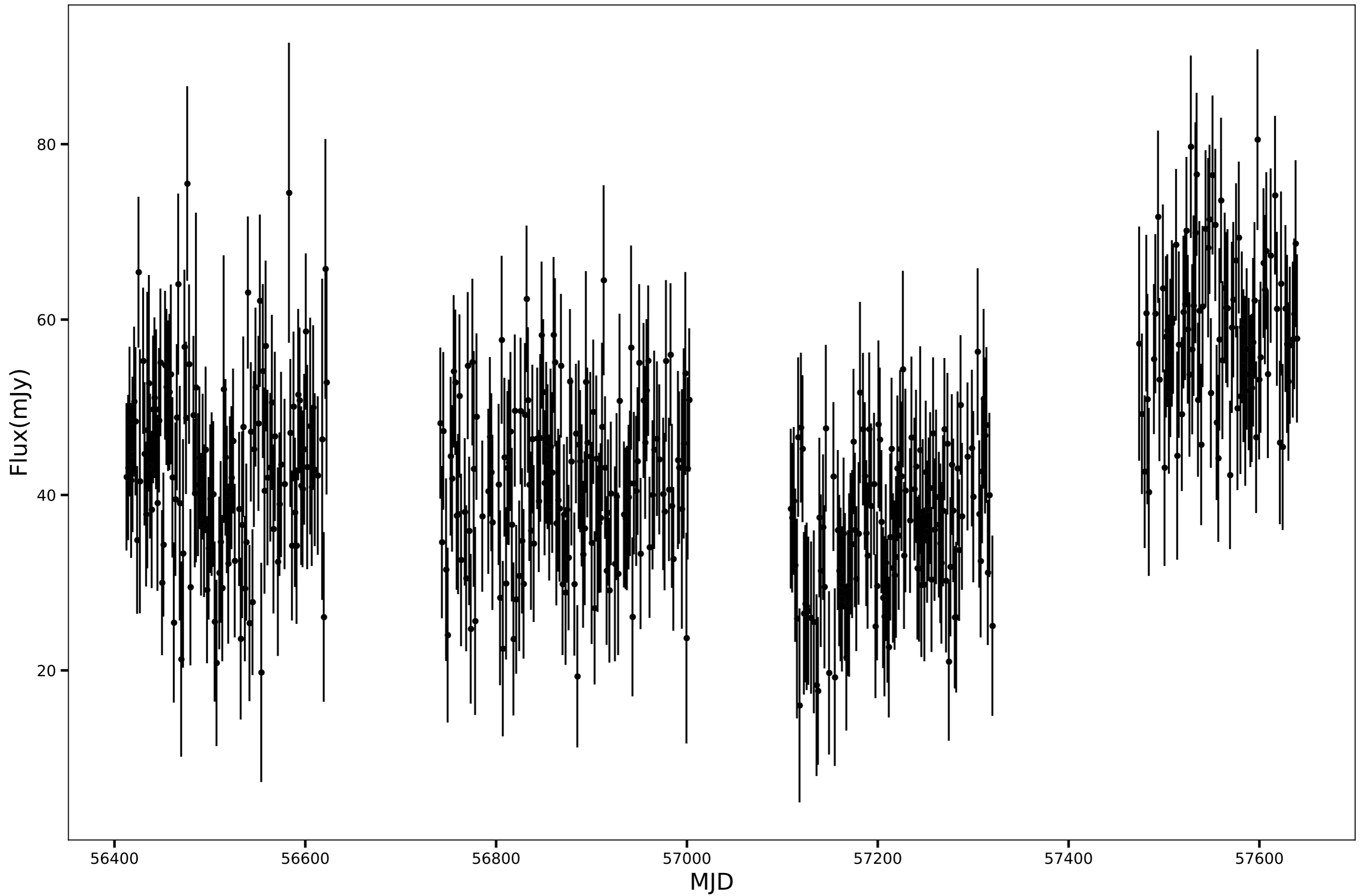
SPT-SJ010406-5657.3, RA=16.0288d, DEC=-56.9554d, mean_flux=43.89 (mJy)
