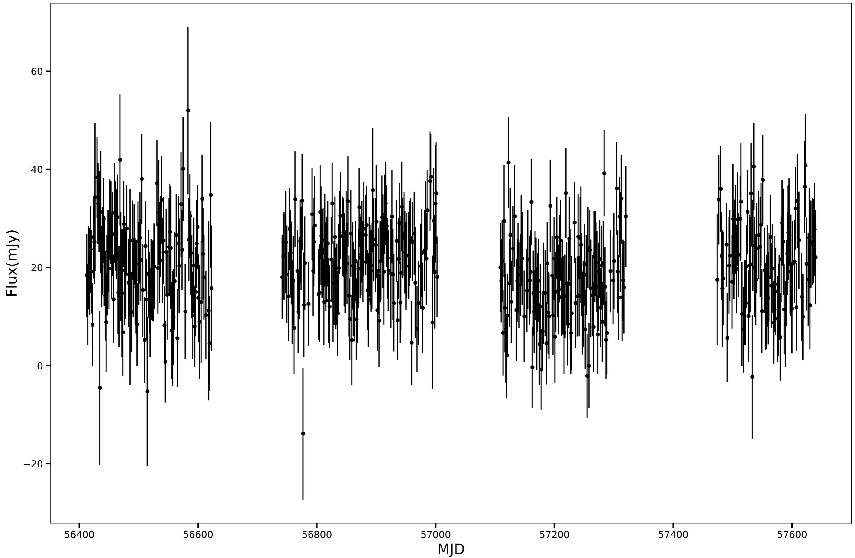
SPT-SJ010350-6351.0, RA=15.9587d, DEC=-63.8511d, mean_flux=19.98 (mJy)
