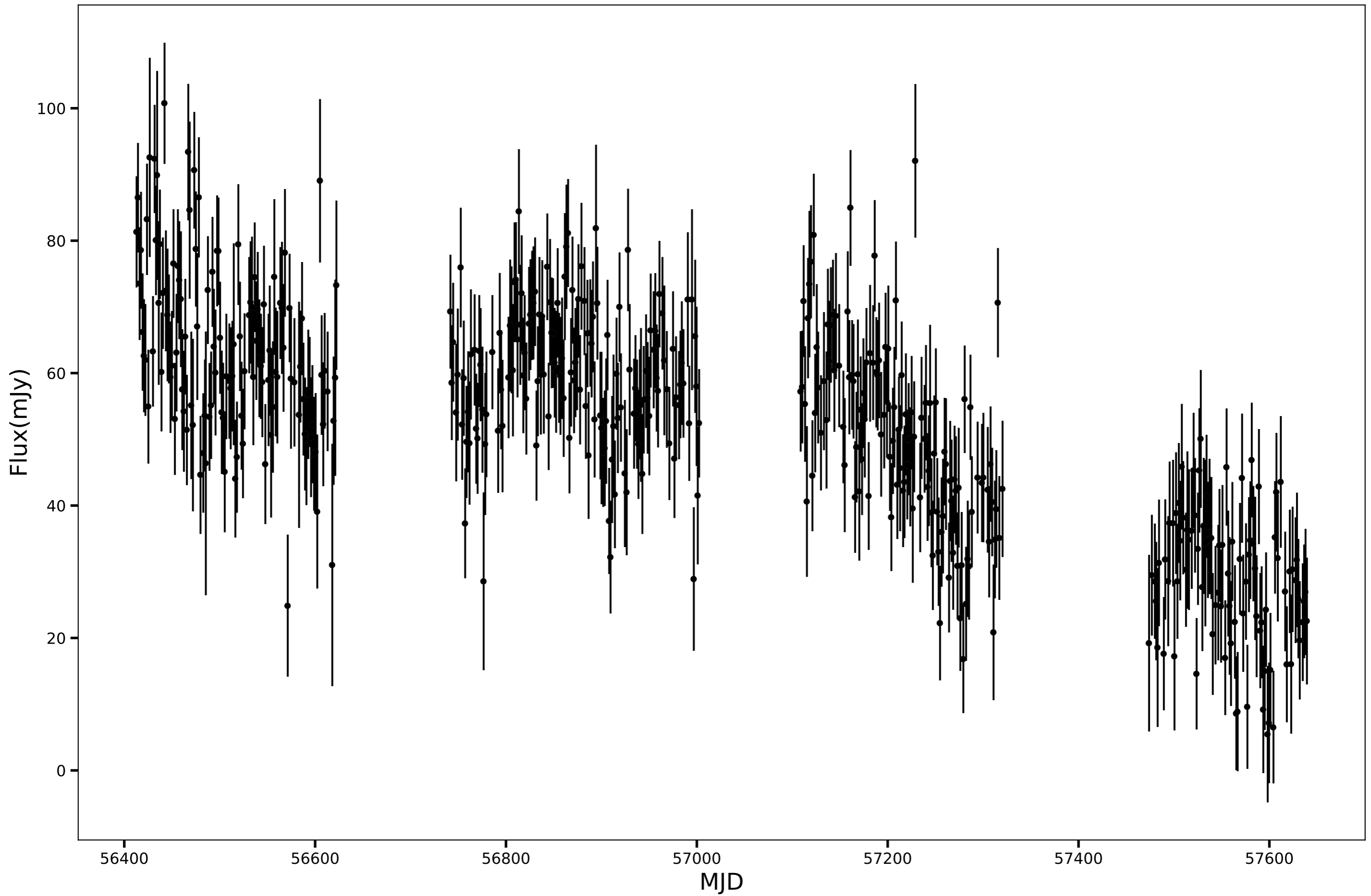
SPT-SJ010306-5109.1, RA=15.7758d, DEC=-51.1525d, mean_flux=52.54 (mJy)
