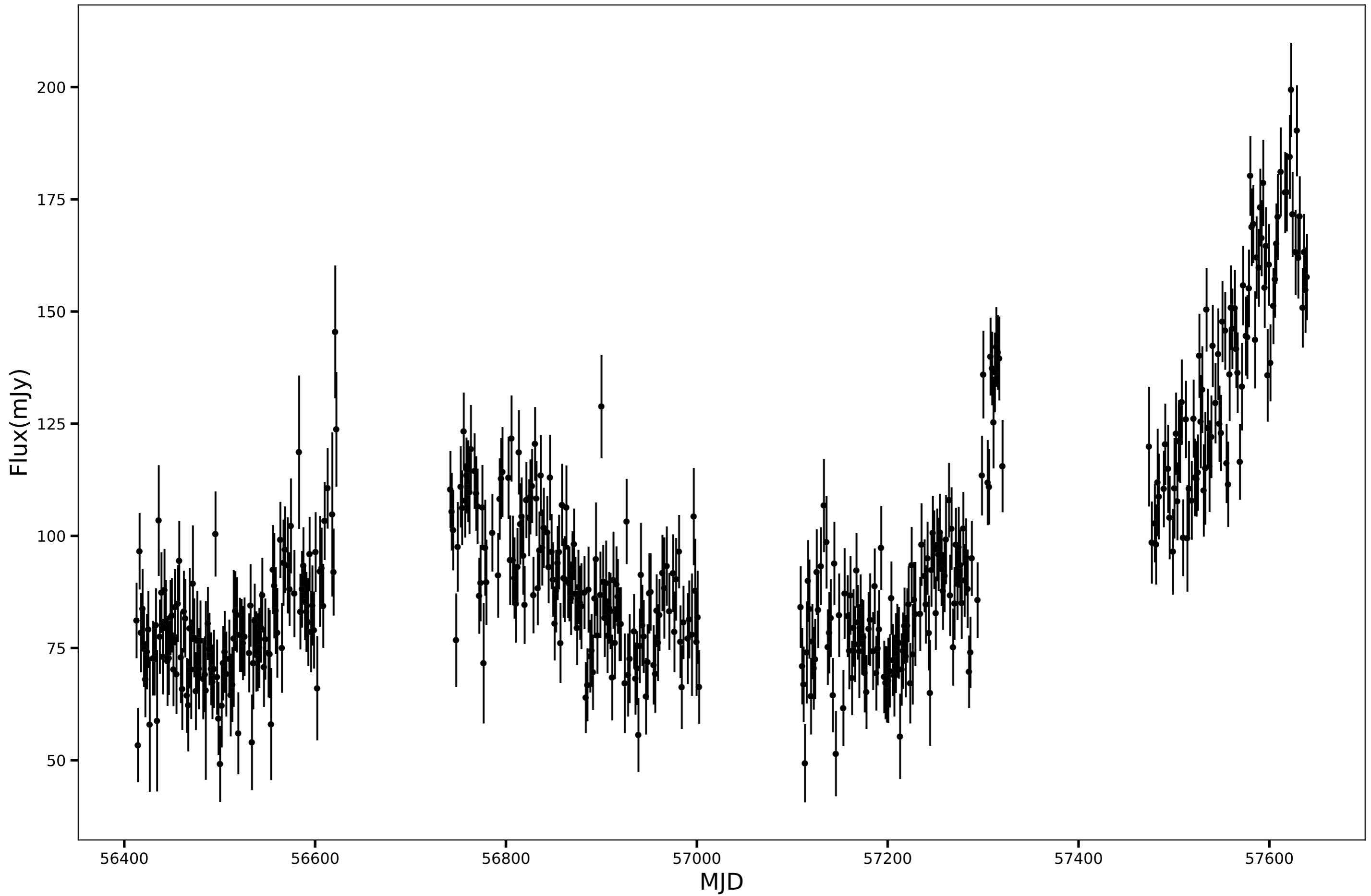
SPT-SJ010210-5637.2, RA=15.5421d, DEC=-56.6204d, mean_flux=96.04 (mJy)
