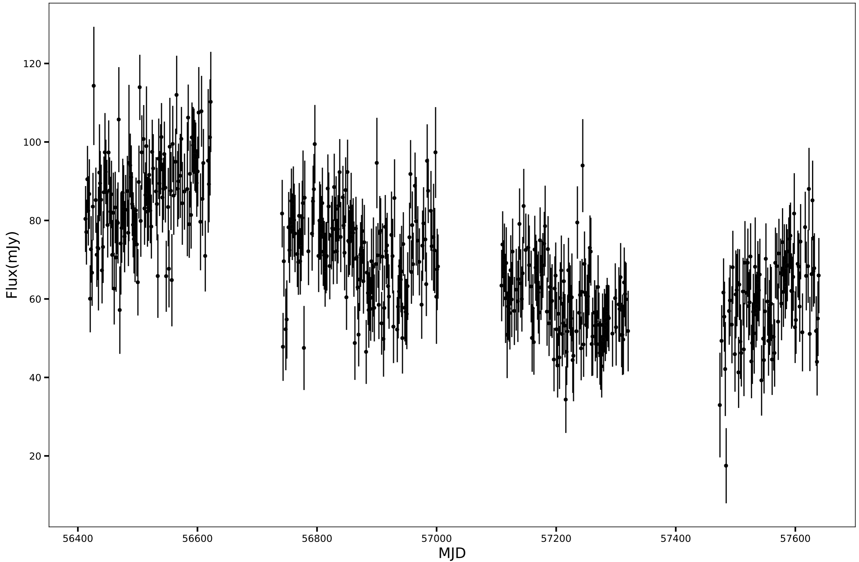
SPT-SJ005856-5219.4, RA=14.7342d, DEC=-52.3244d, mean_flux=70.24 (mJy)
