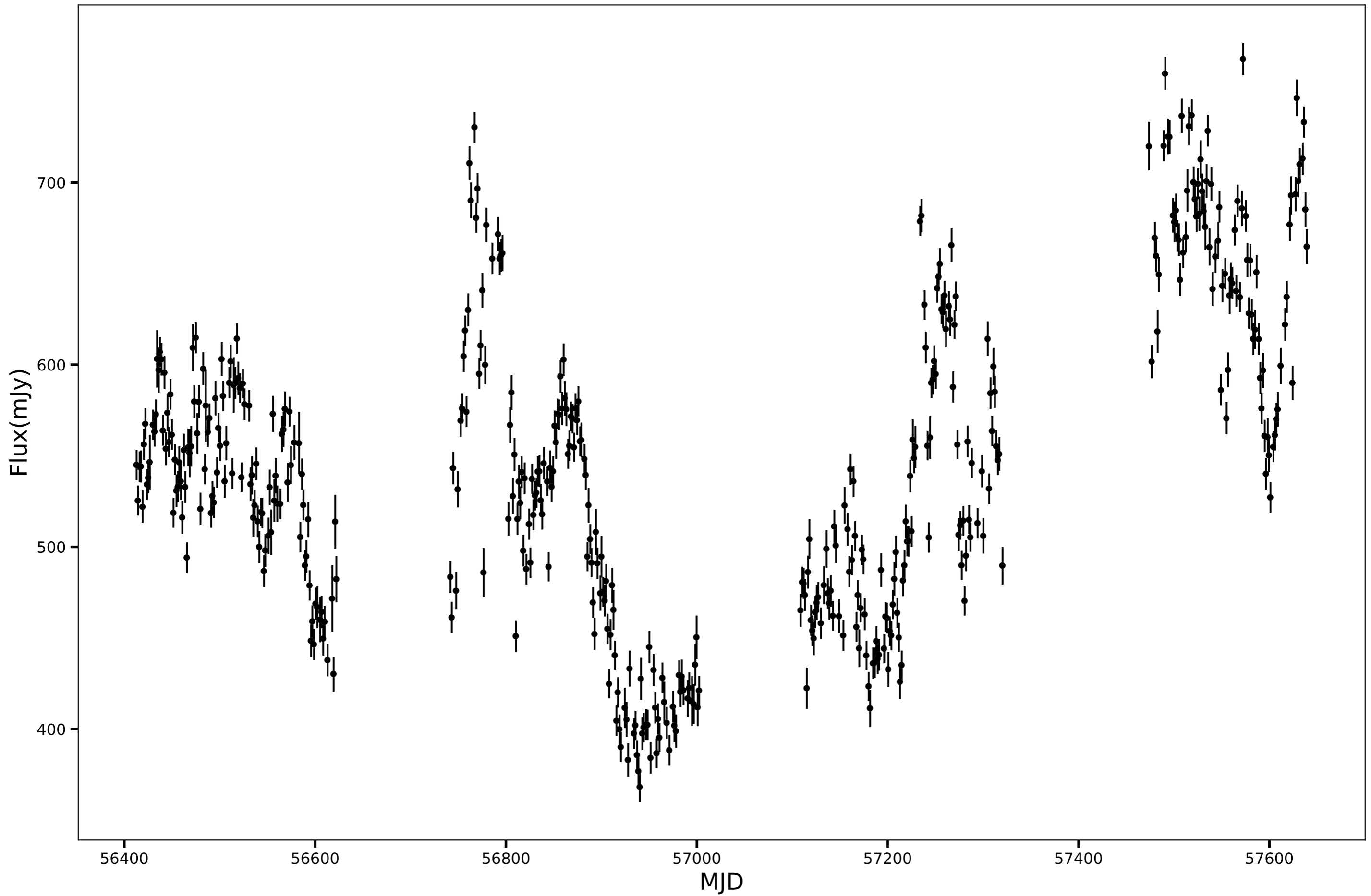
SPT-SJ005846-5659.1, RA=14.6944d, DEC=-56.9855d, mean_flux=546.05 (mJy)
