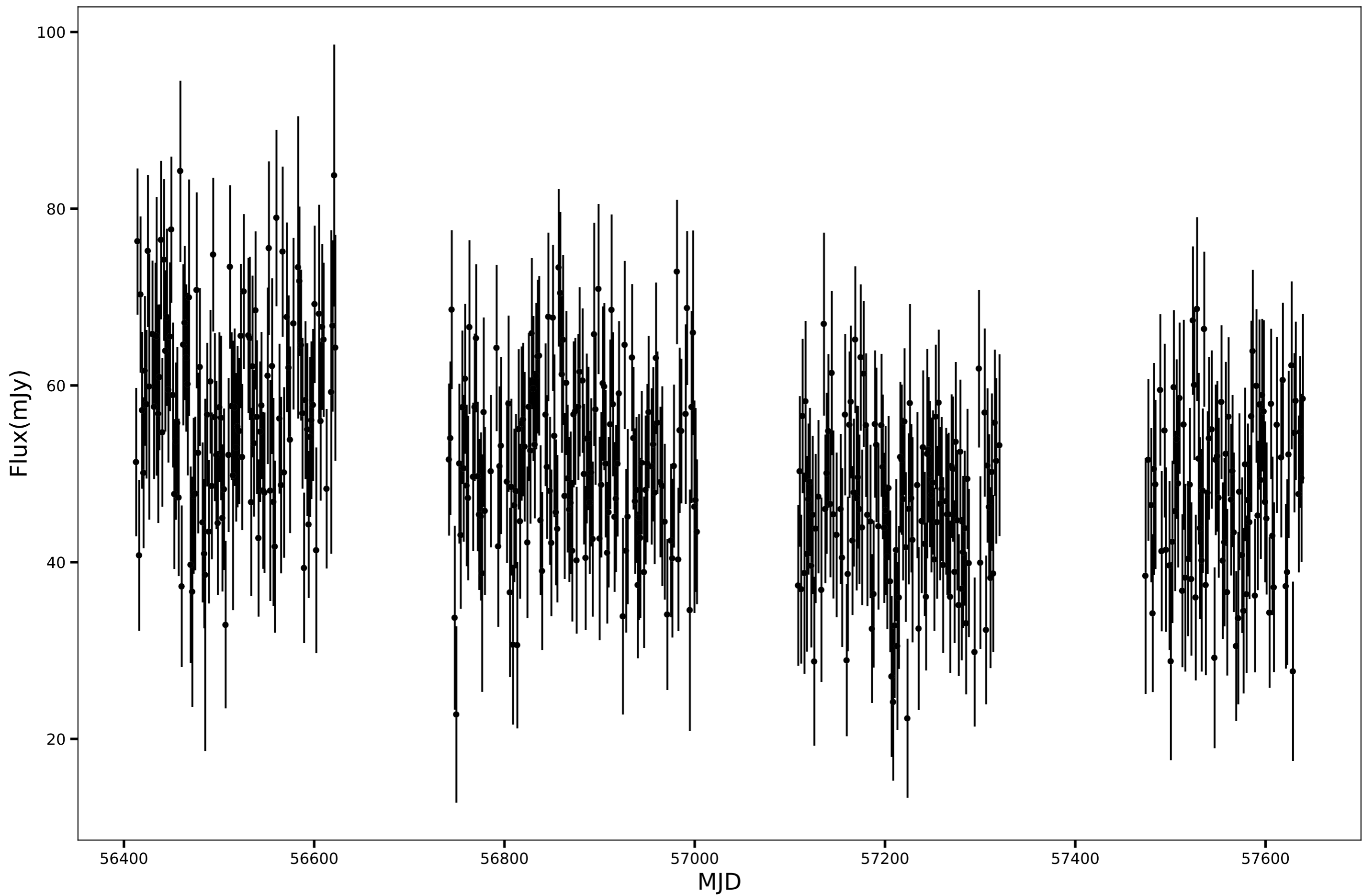
SPT-SJ005705-5214.3, RA=14.2738d, DEC=-52.2392d, mean_flux=51.06 (mJy)
