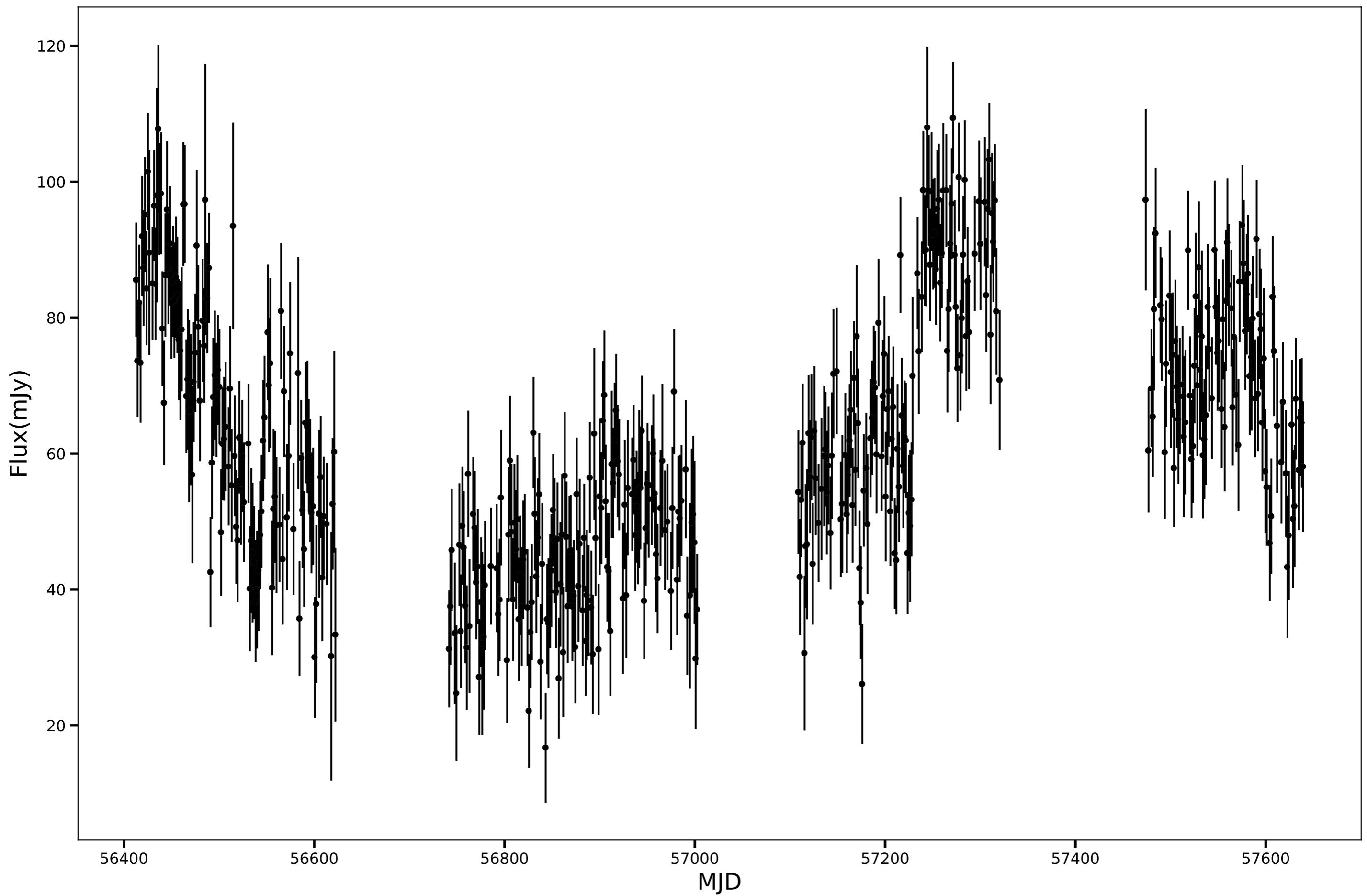
SPT-SJ004905-5521.1, RA=12.2742d, DEC=-55.3524d, mean_flux=62.20 (mJy)
