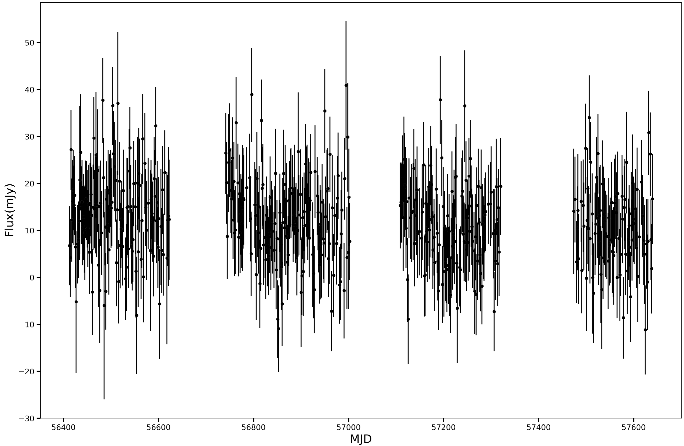
SPT-SJ003813-6112.8, RA=9.5554d, DEC=-61.2139d, mean_flux=11.92 (mJy)
