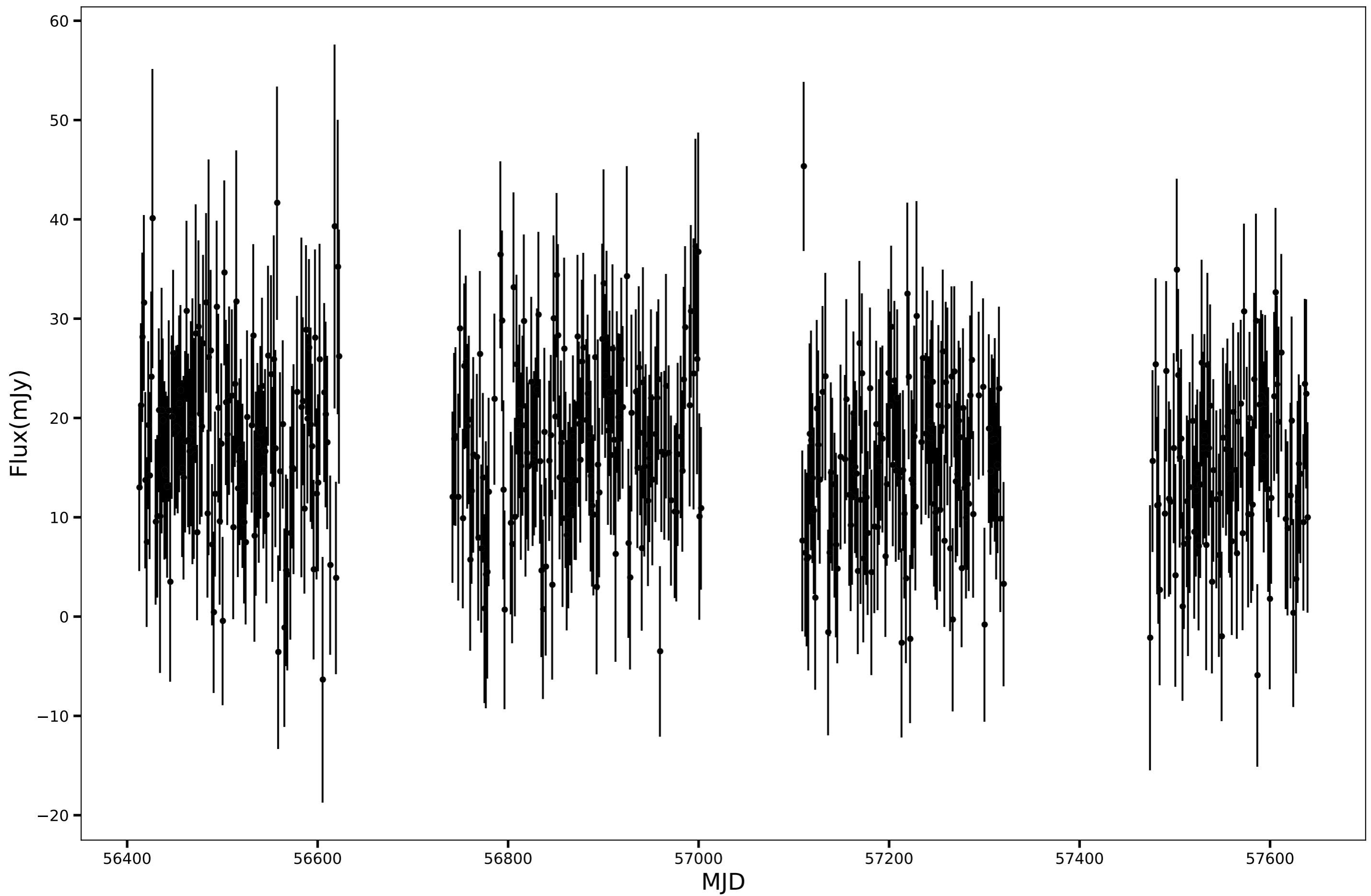
SPT-SJ003725-5917.9, RA=9.3572d, DEC=-59.2997d, mean_flux=16.56 (mJy)
