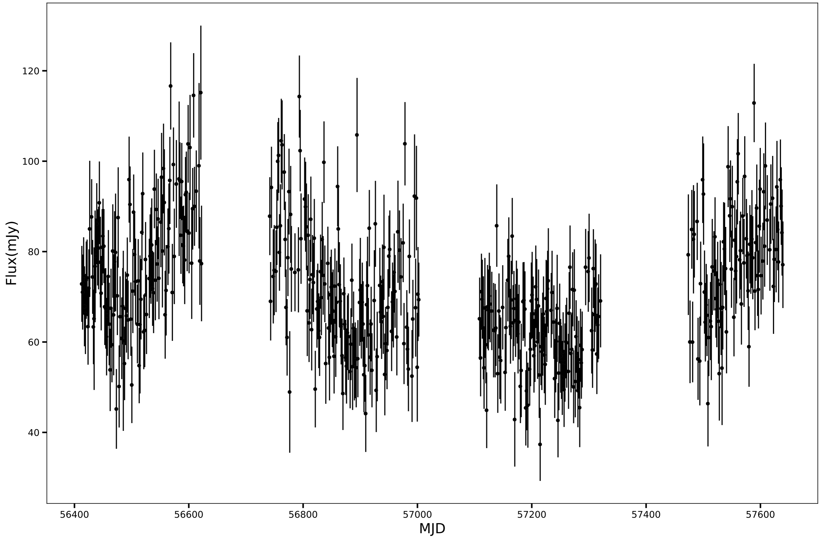
SPT-SJ003133-5143.3, RA=7.8913d, DEC=-51.7229d, mean_flux=72.14 (mJy)
